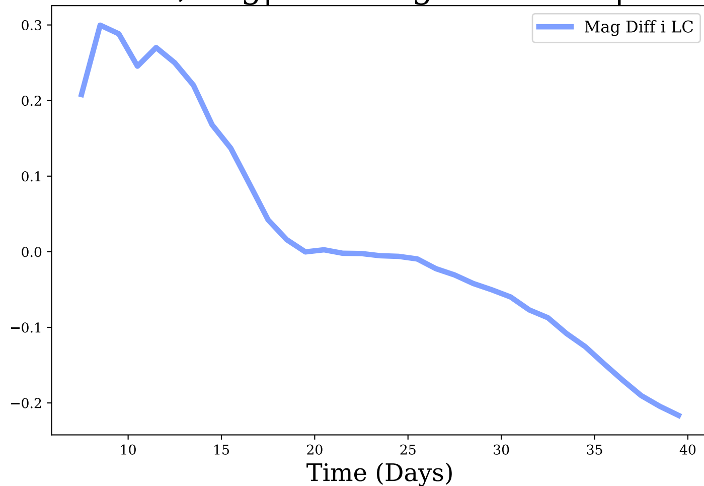
i-band, Avg|Max Mag Diff: 0.02 | 0.3
