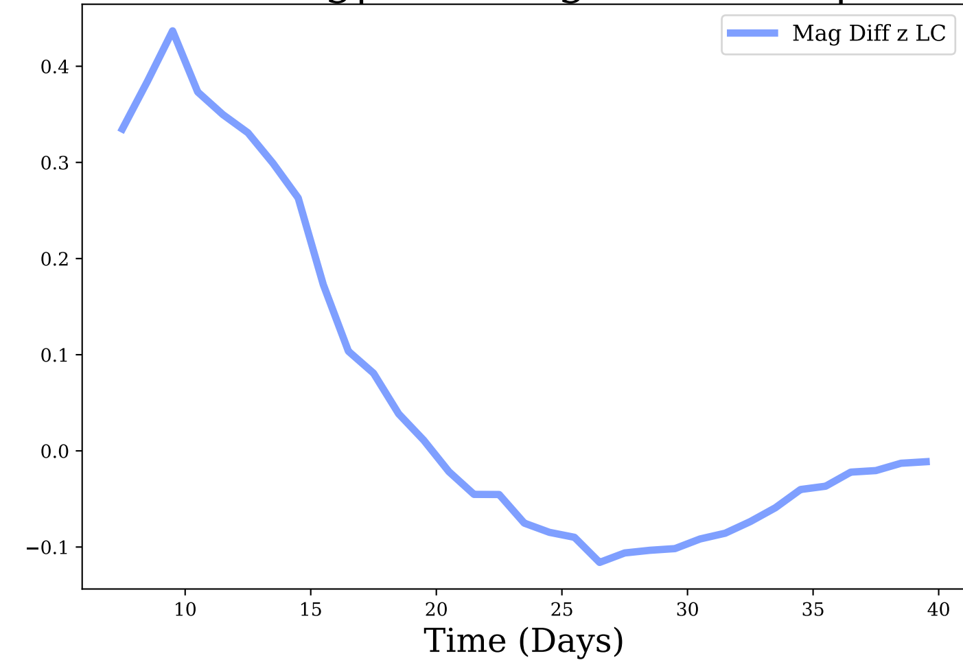
z-band, Avg|Max Mag Diff: 0.06 | 0.44
