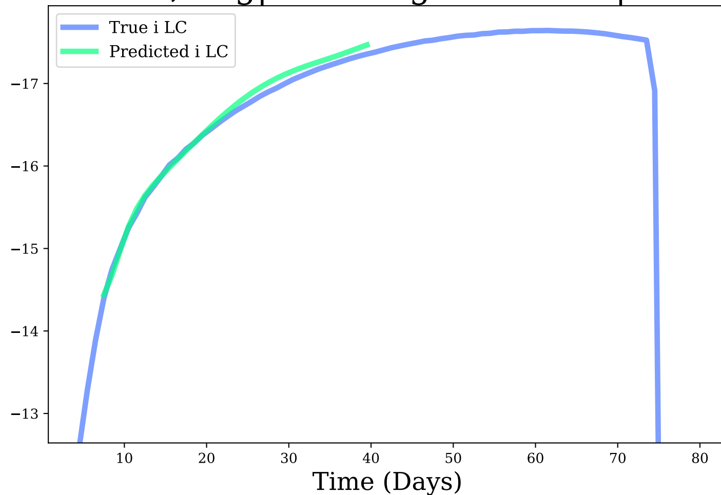
i-band, Avg|Max Mag Diff: 0.06 | 0.12
