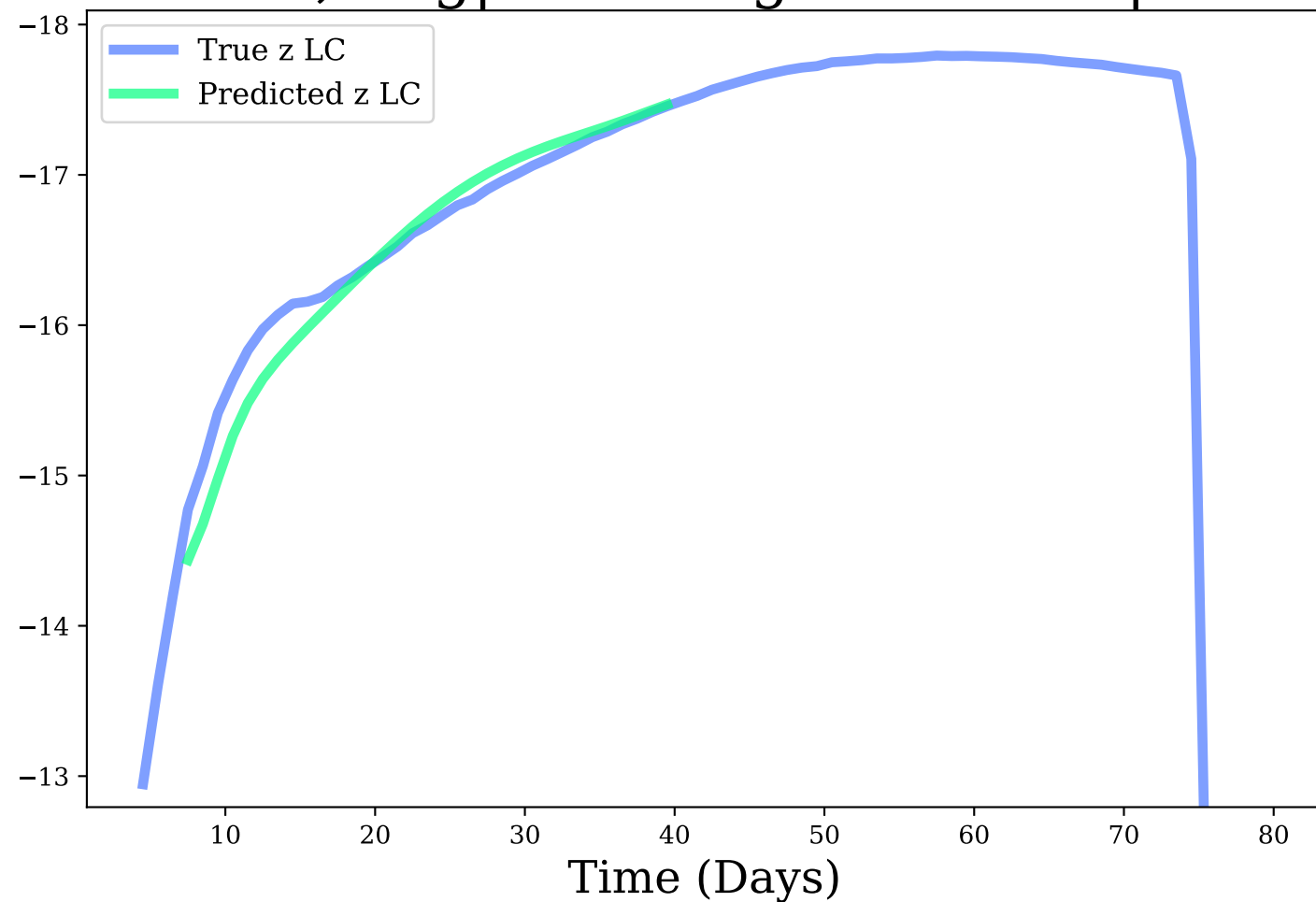
z-band, Avg|Max Mag Diff: 0.13 | 0.44
