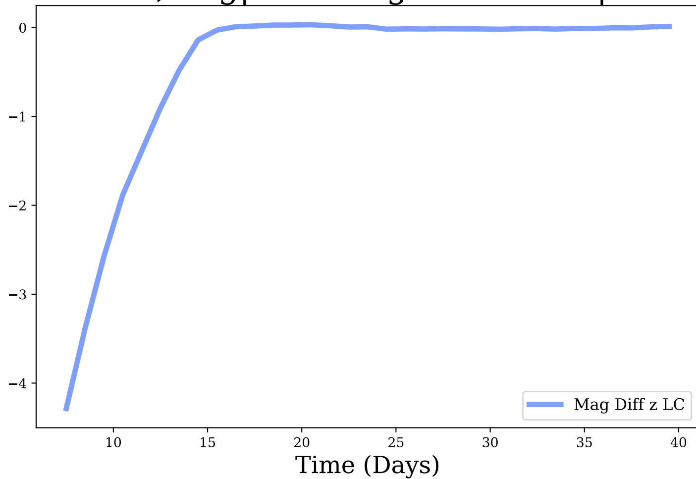
z-band, Avg|Max Mag Diff: -0.46 | 4.29
