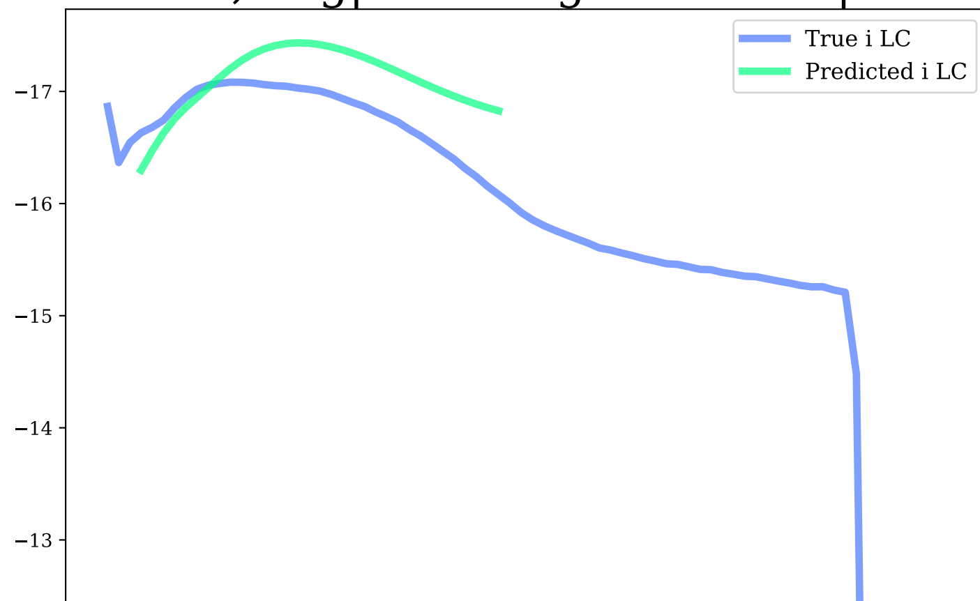
i-band, Avg|Max Mag Diff: 0.37 | 0.75
