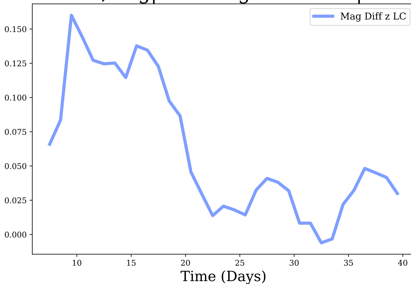
z-band, Avg|Max Mag Diff: 0.06 | 0.16
