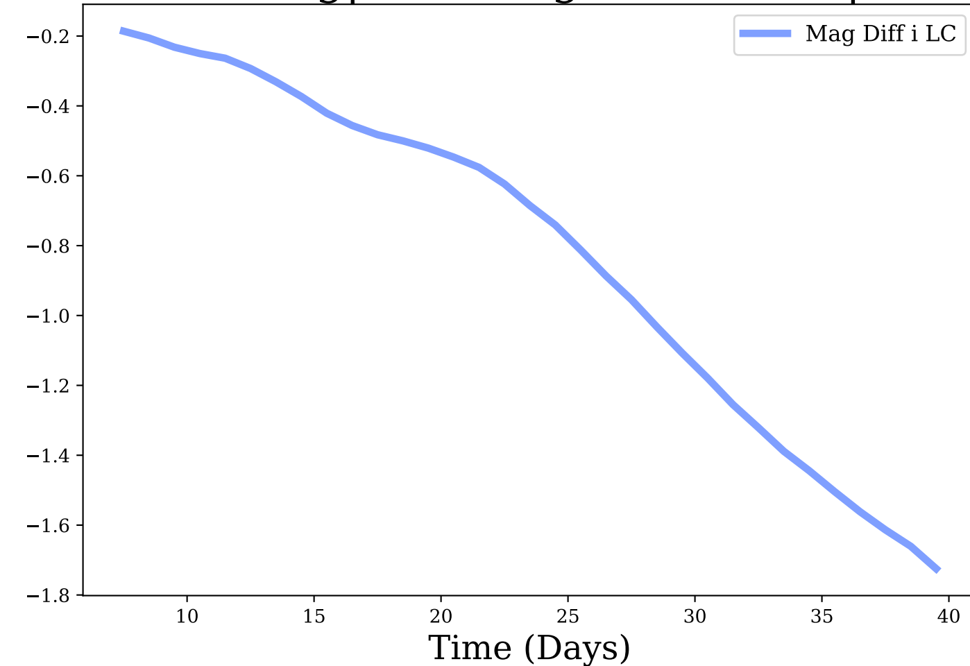
i-band, Avg|Max Mag Diff: -0.82 | 1.72
