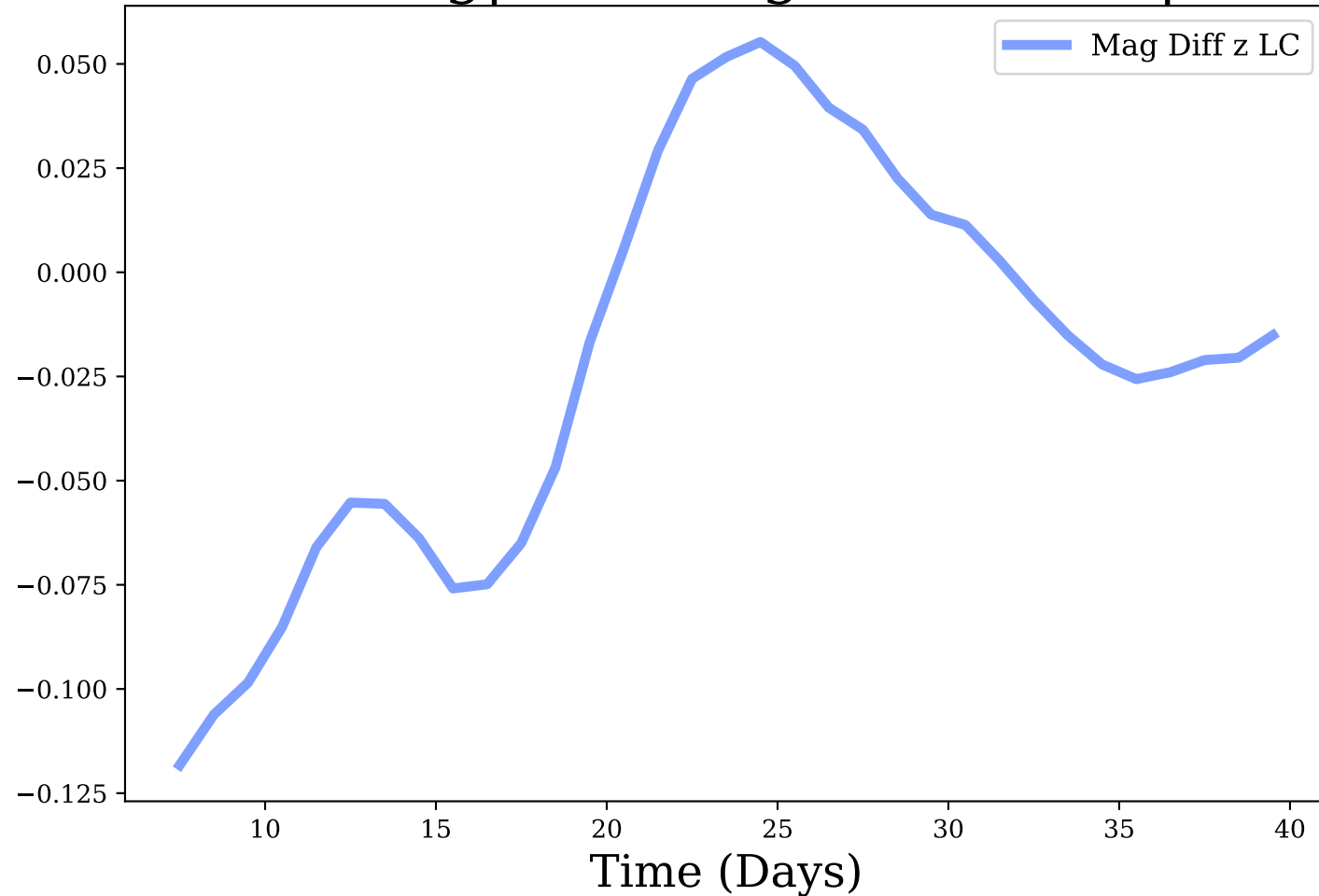
z-band, Avg|Max Mag Diff: -0.02 | 0.12
