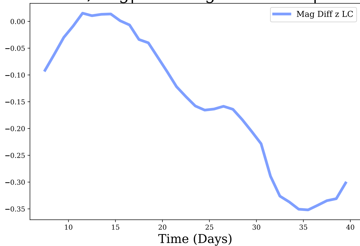
z-band, Avg|Max Mag Diff: -0.15 | 0.35
