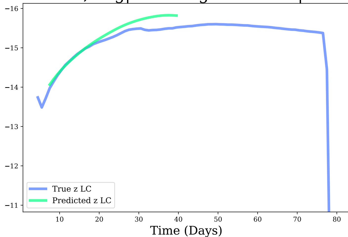
z-band, Avg|Max Mag Diff: 0.16 | 0.35
