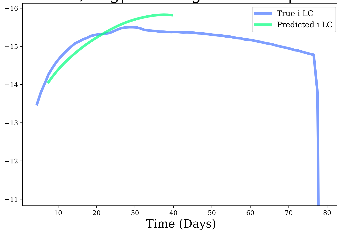
i-band, Avg|Max Mag Diff: 0.23 | 0.45
