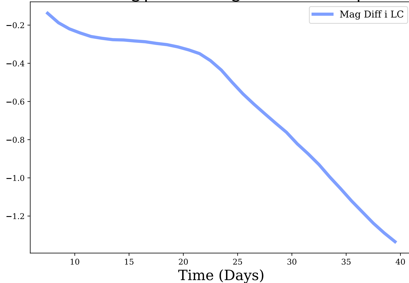
i-band, Avg|Max Mag Diff: -0.59 | 1.33
