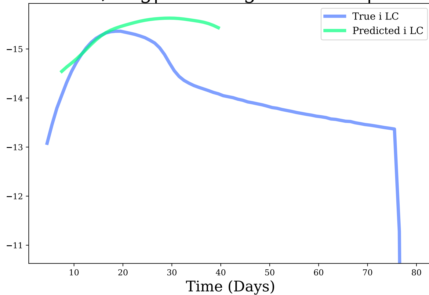
i-band, Avg|Max Mag Diff: 0.57 | 1.37
