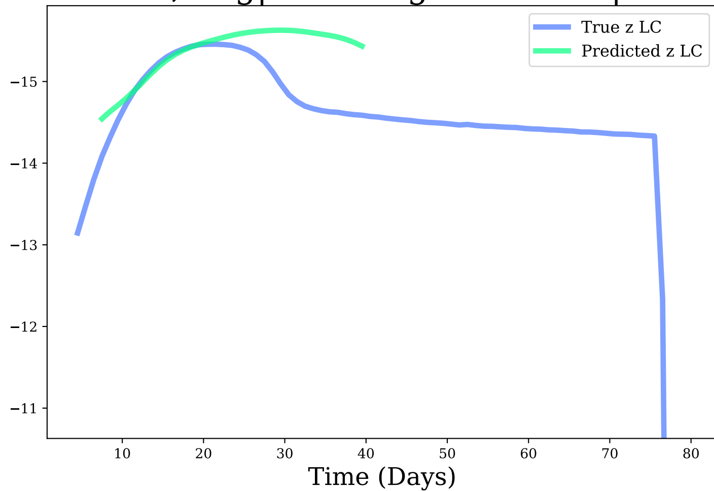
z-band, Avg|Max Mag Diff: 0.38 | 0.94
