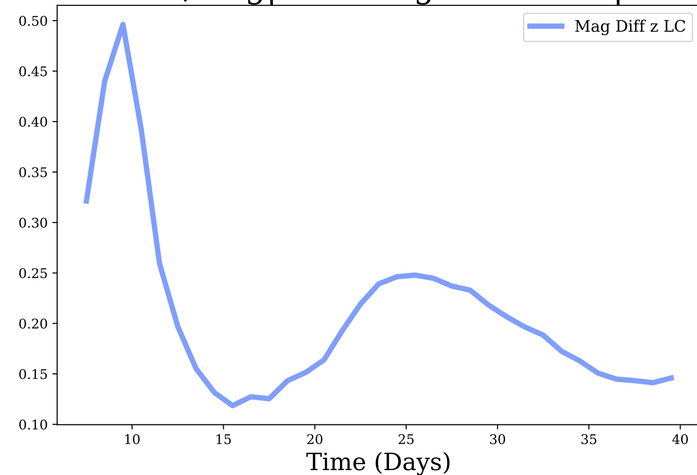
z-band, Avg|Max Mag Diff: 0.21 | 0.5
