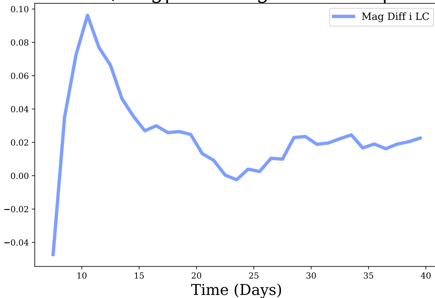
i-band, Avg|Max Mag Diff: 0.02 | 0.1
