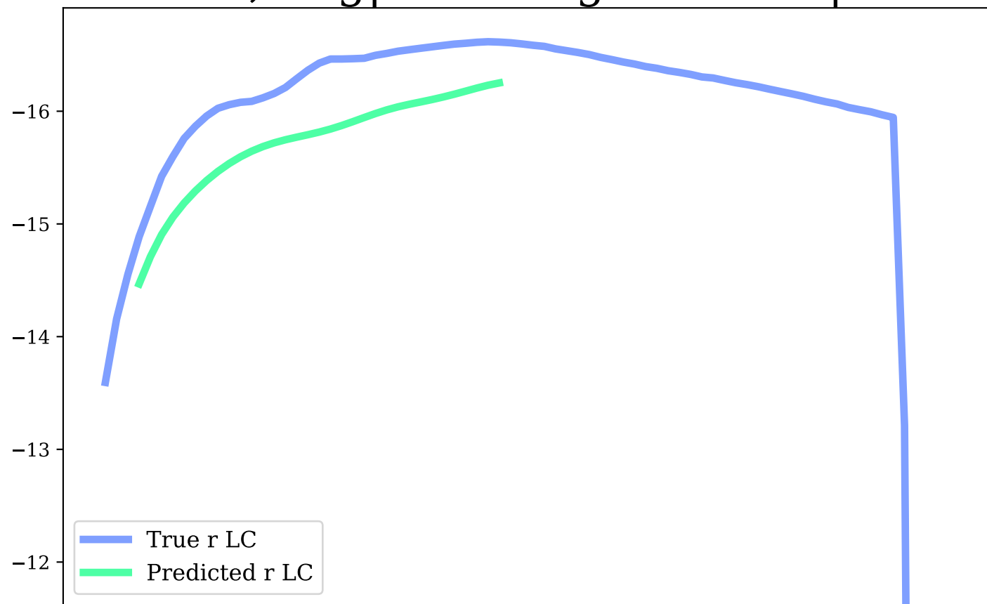
z-band, Avg|Max Mag Diff: 0.08 | 0.21
