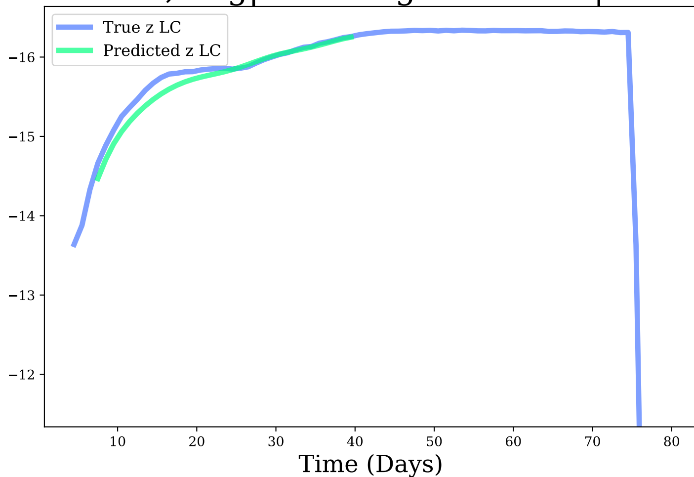
z-band, Avg|Max Mag Diff: 0.08 | 0.21
