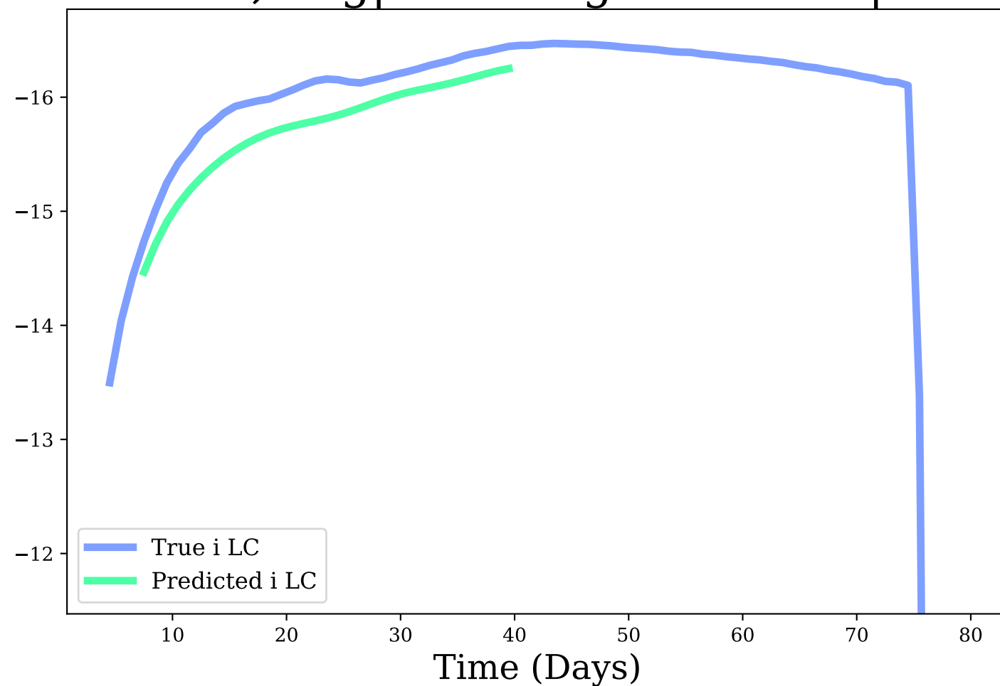
i-band, Avg|Max Mag Diff: 0.28 | 0.4
