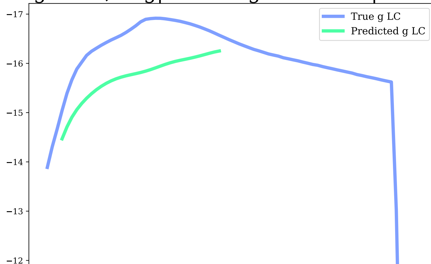
i-band, Avg|Max Mag Diff: 0.28 | 0.4
