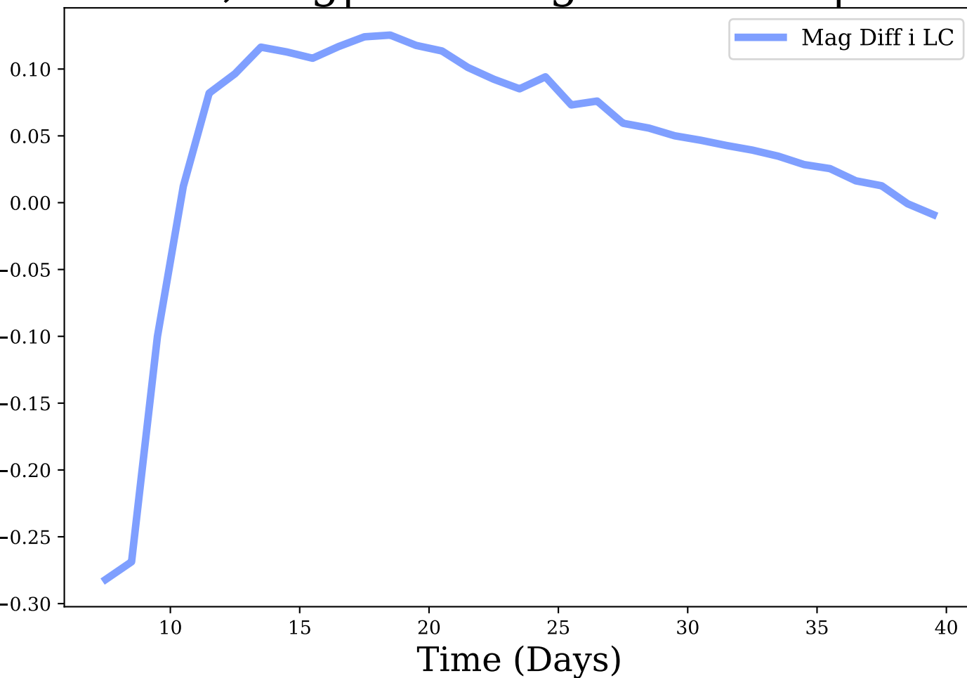
i-band, Avg|Max Mag Diff: 0.04 | 0.28
