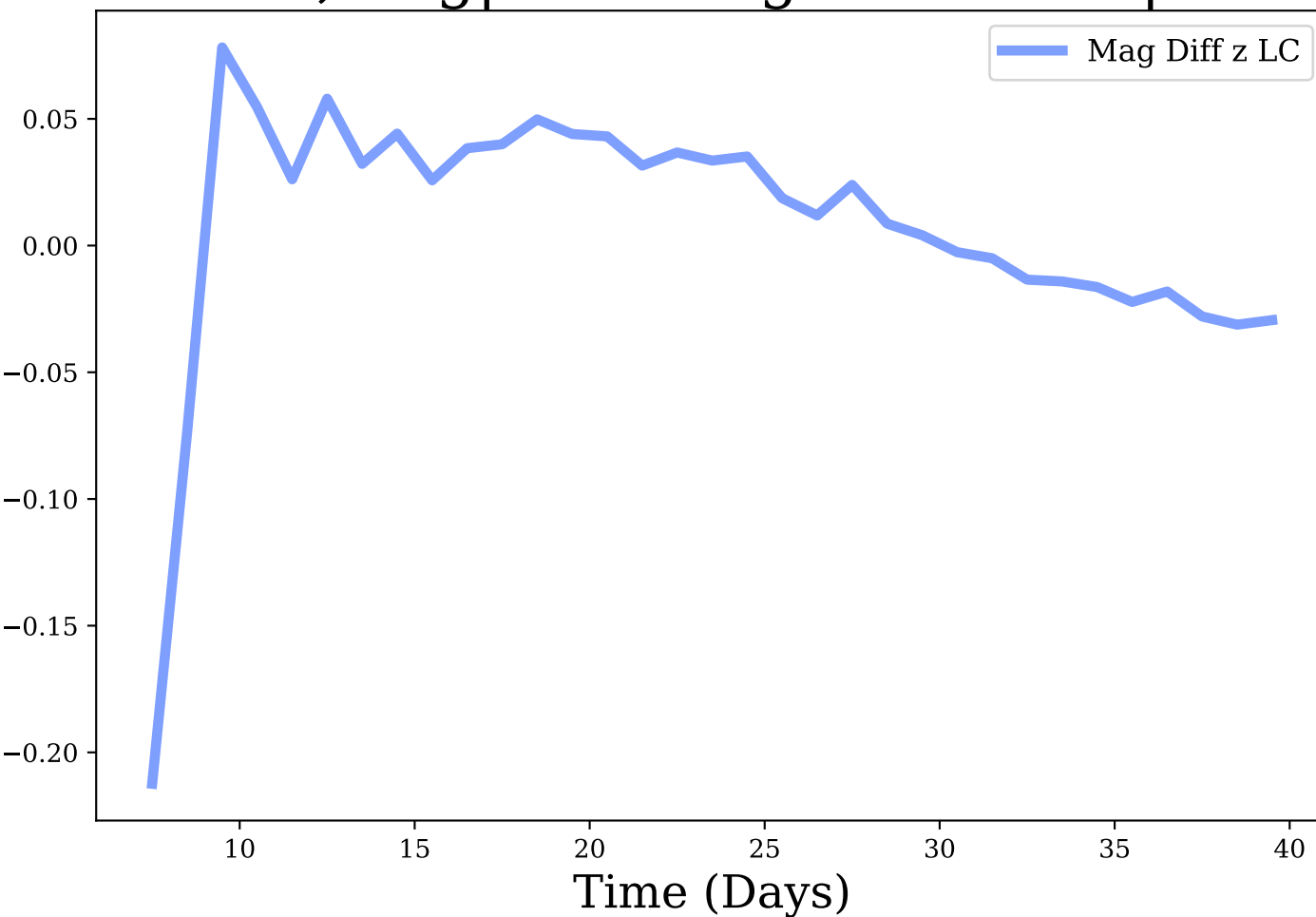
z-band, Avg|Max Mag Diff: 0.01 | 0.21
