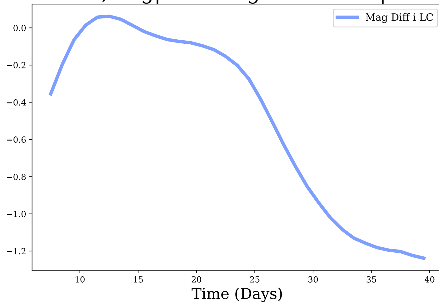
i-band, Avg|Max Mag Diff: -0.49 | 1.24
