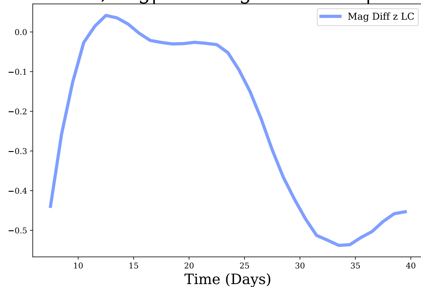
z-band, Avg|Max Mag Diff: -0.23 | 0.54
