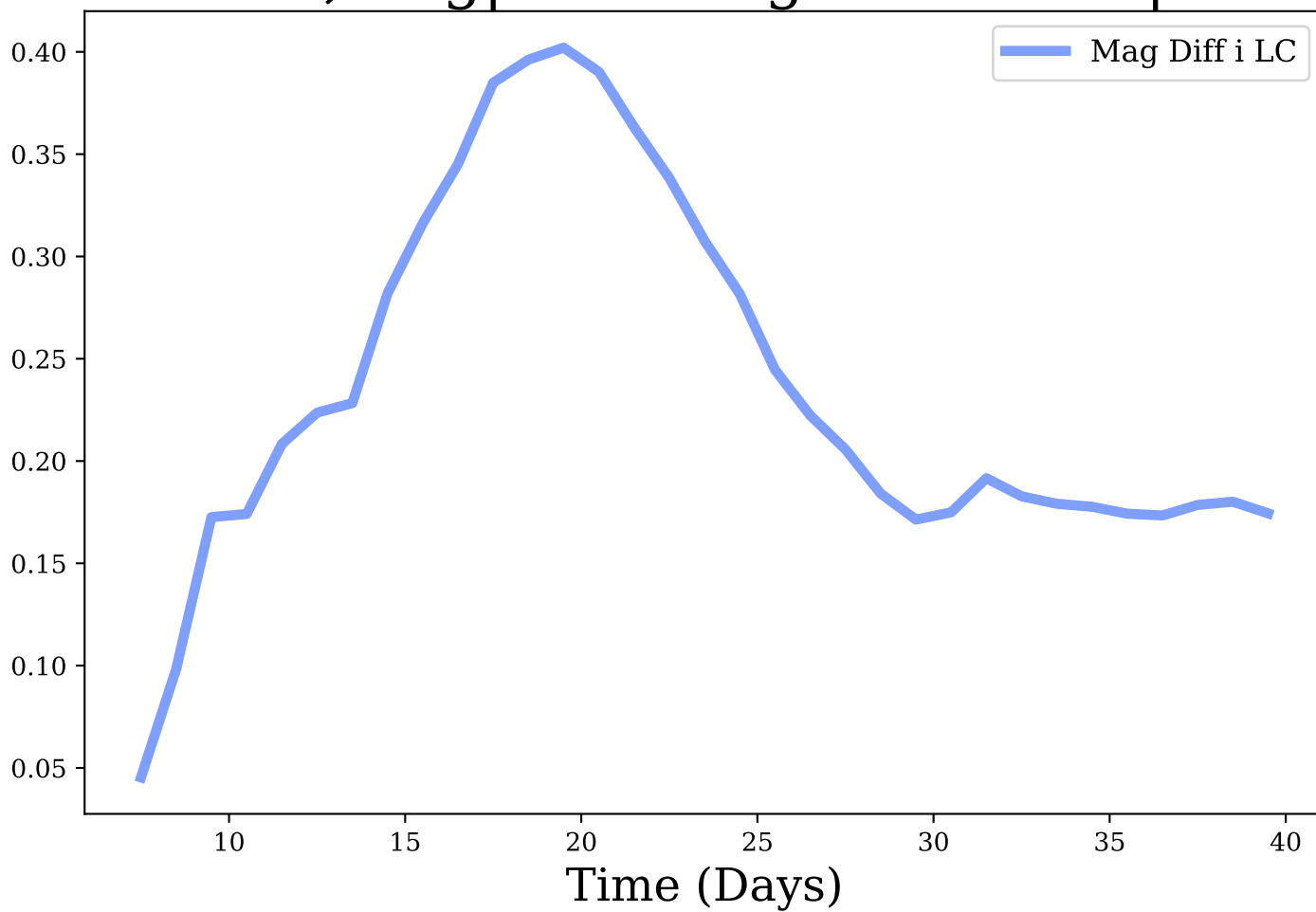
i-band, Avg|Max Mag Diff: 0.24 | 0.4
