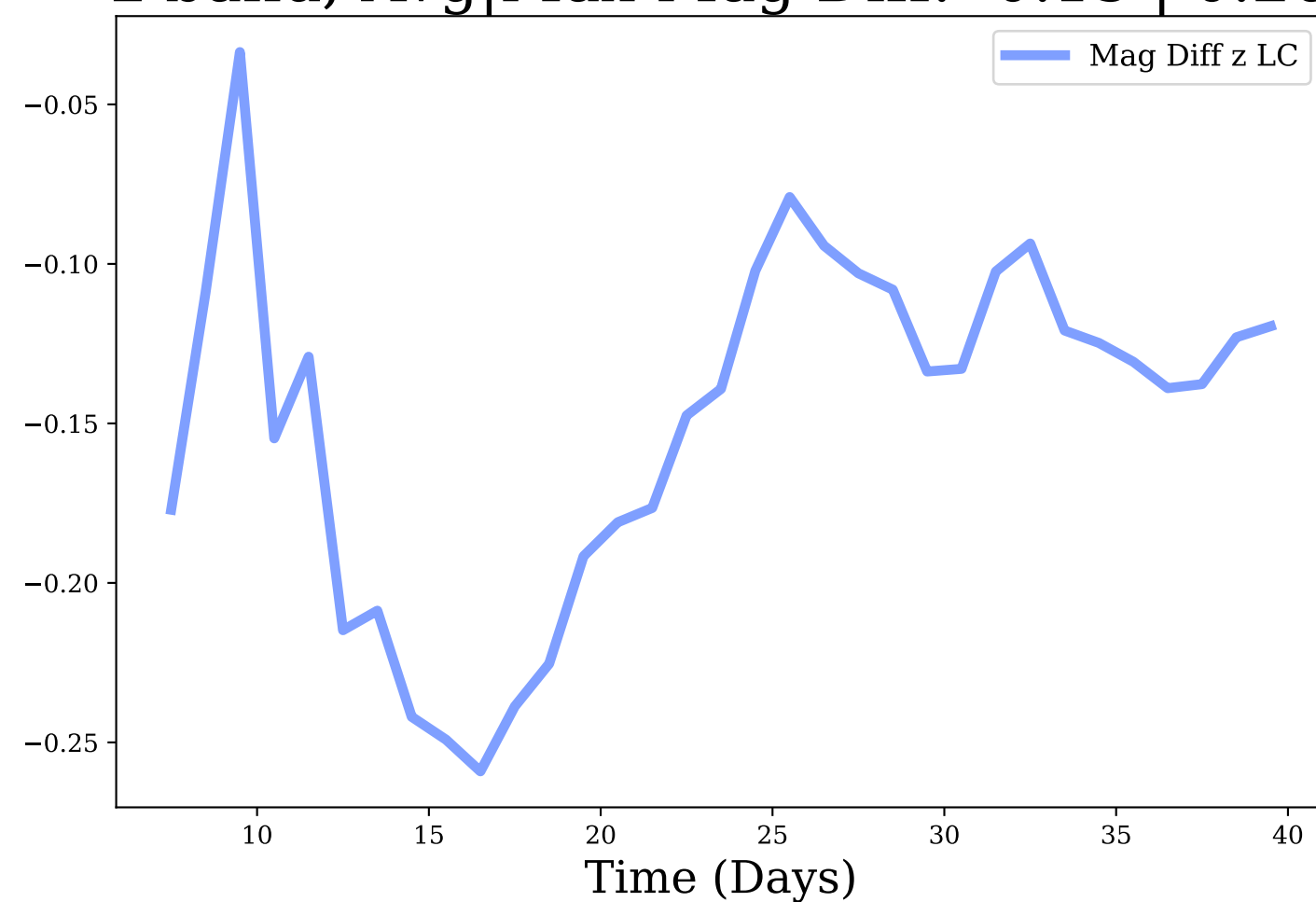
z-band, Avg|Max Mag Diff: -0.15 | 0.26
