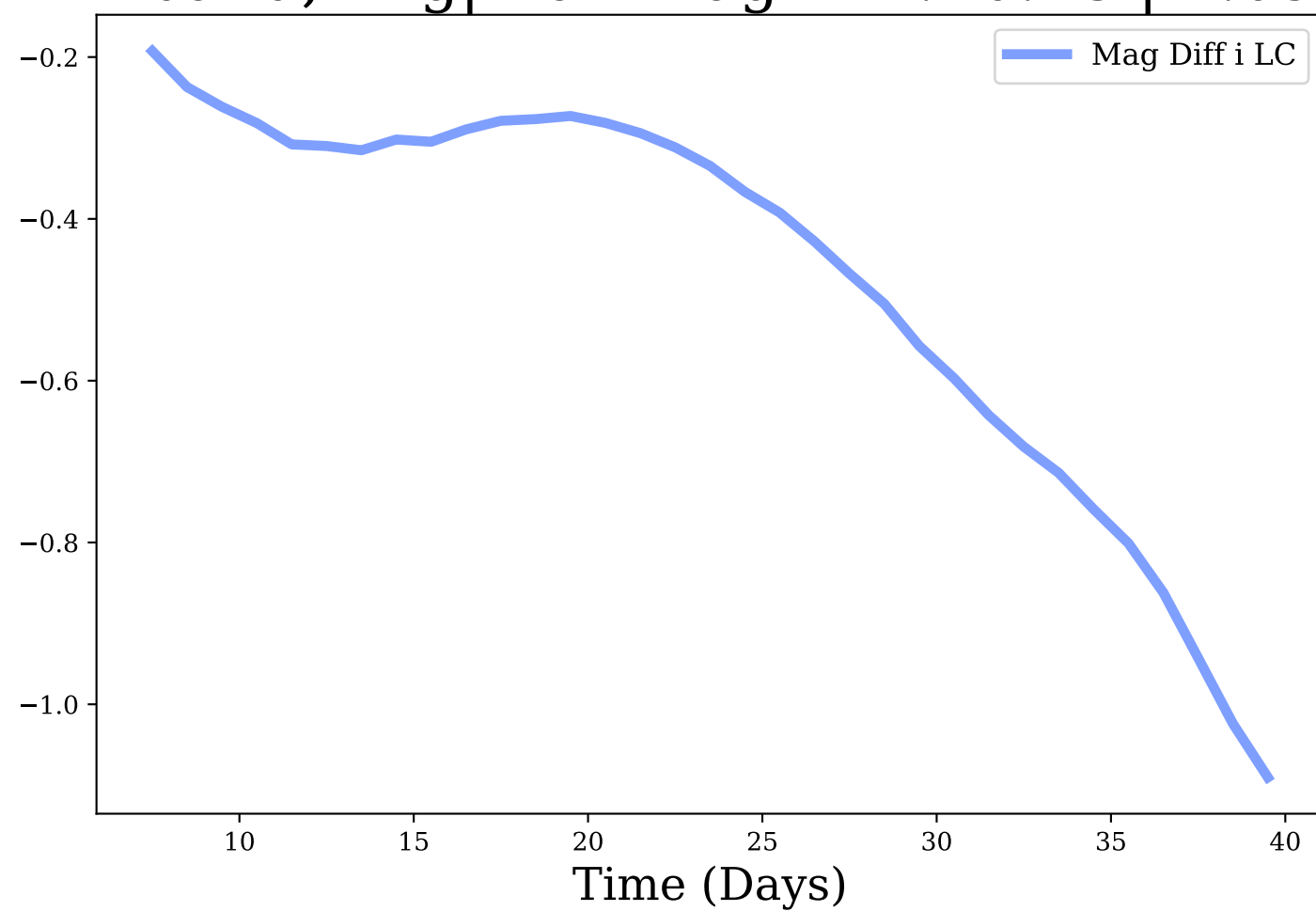
i-band, Avg|Max Mag Diff: -0.48 | 1.09
