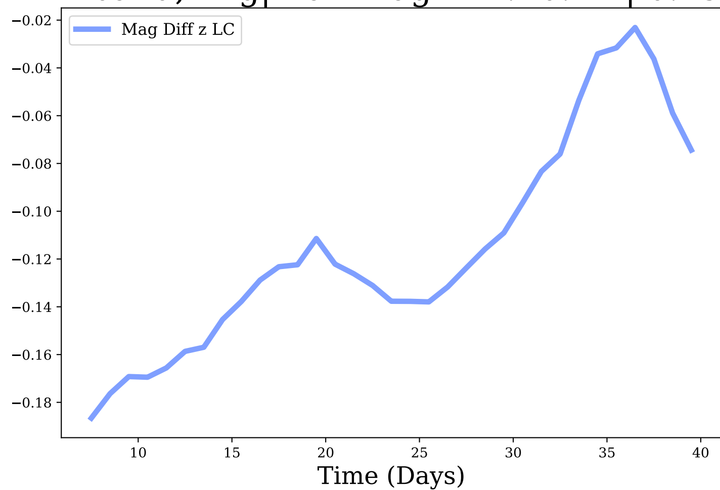
z-band, Avg|Max Mag Diff: -0.11 | 0.19
