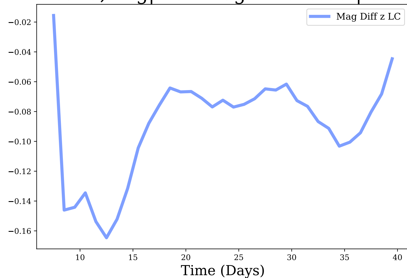
z-band, Avg|Max Mag Diff: -0.09 | 0.16
