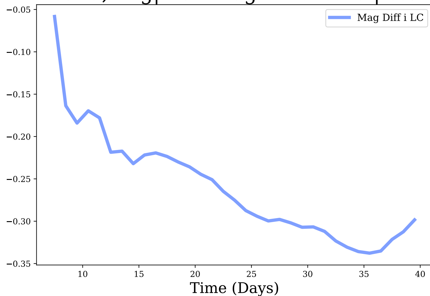
i-band, Avg|Max Mag Diff: -0.26 | 0.34
