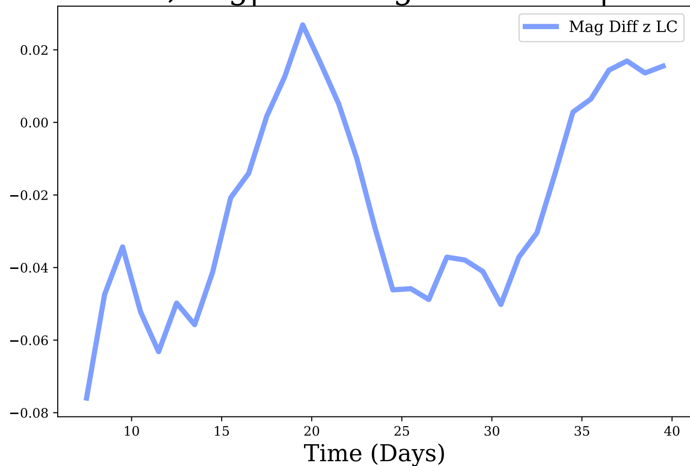
z-band, Avg|Max Mag Diff: -0.02 | 0.08
