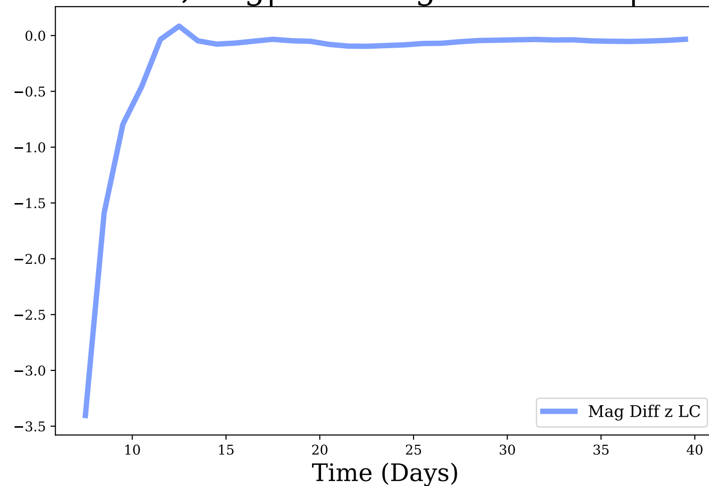
z-band, Avg|Max Mag Diff: -0.23 | 3.4
