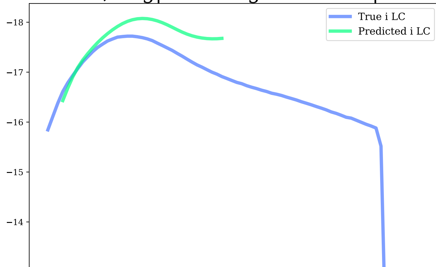
i-band, Avg|Max Mag Diff: 0.35 | 0.77
