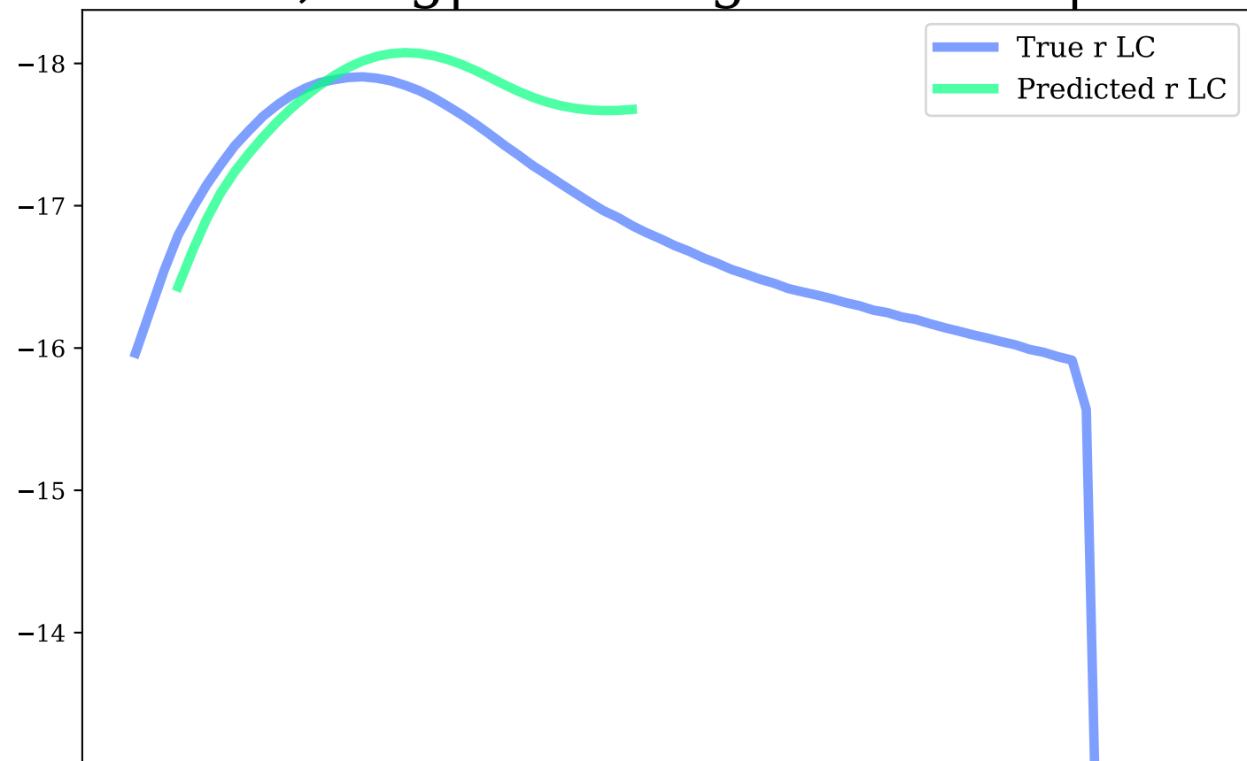
z-band, Avg|Max Mag Diff: 0.08 | 0.22
