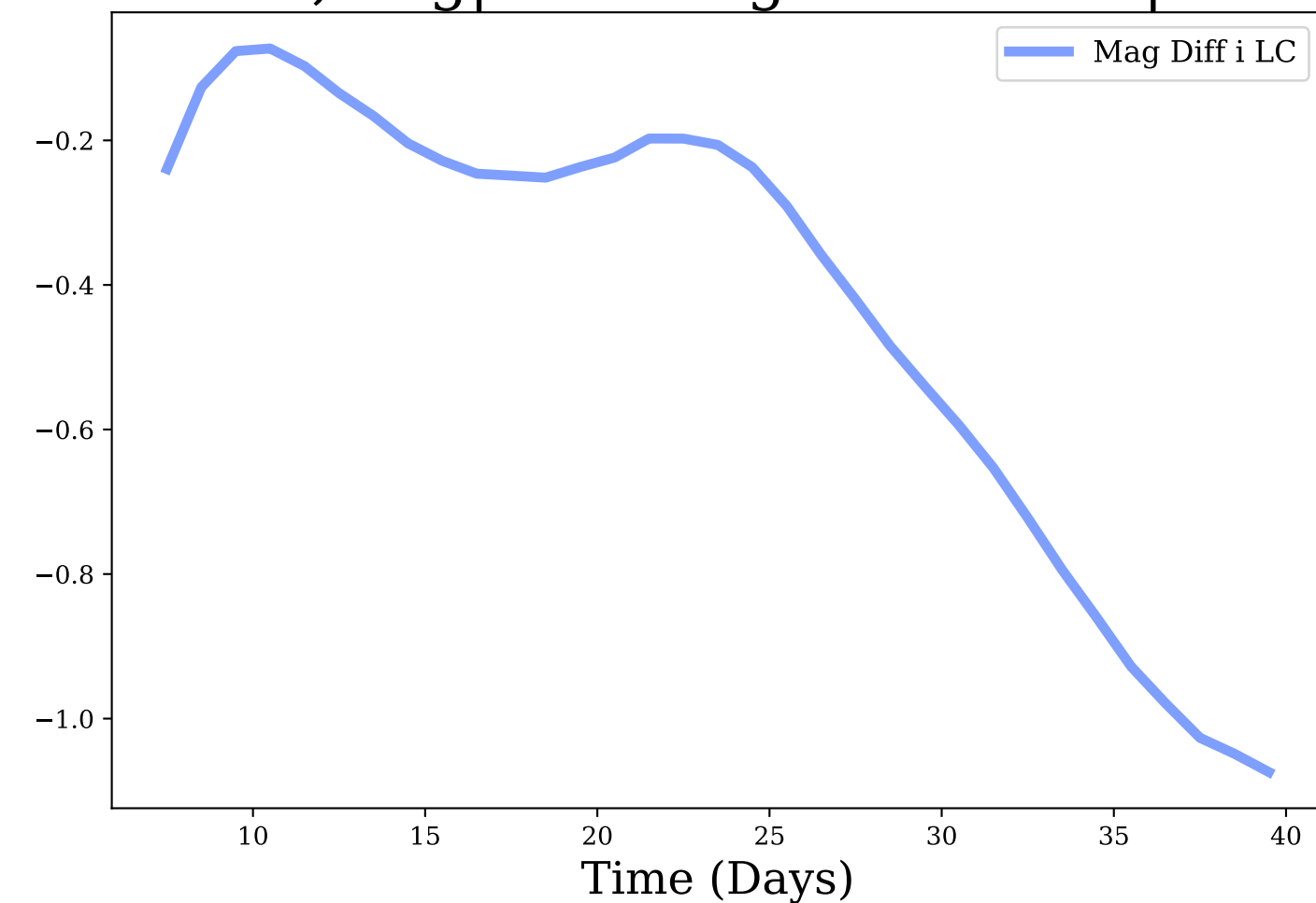
i-band, Avg|Max Mag Diff: -0.43 | 1.07
