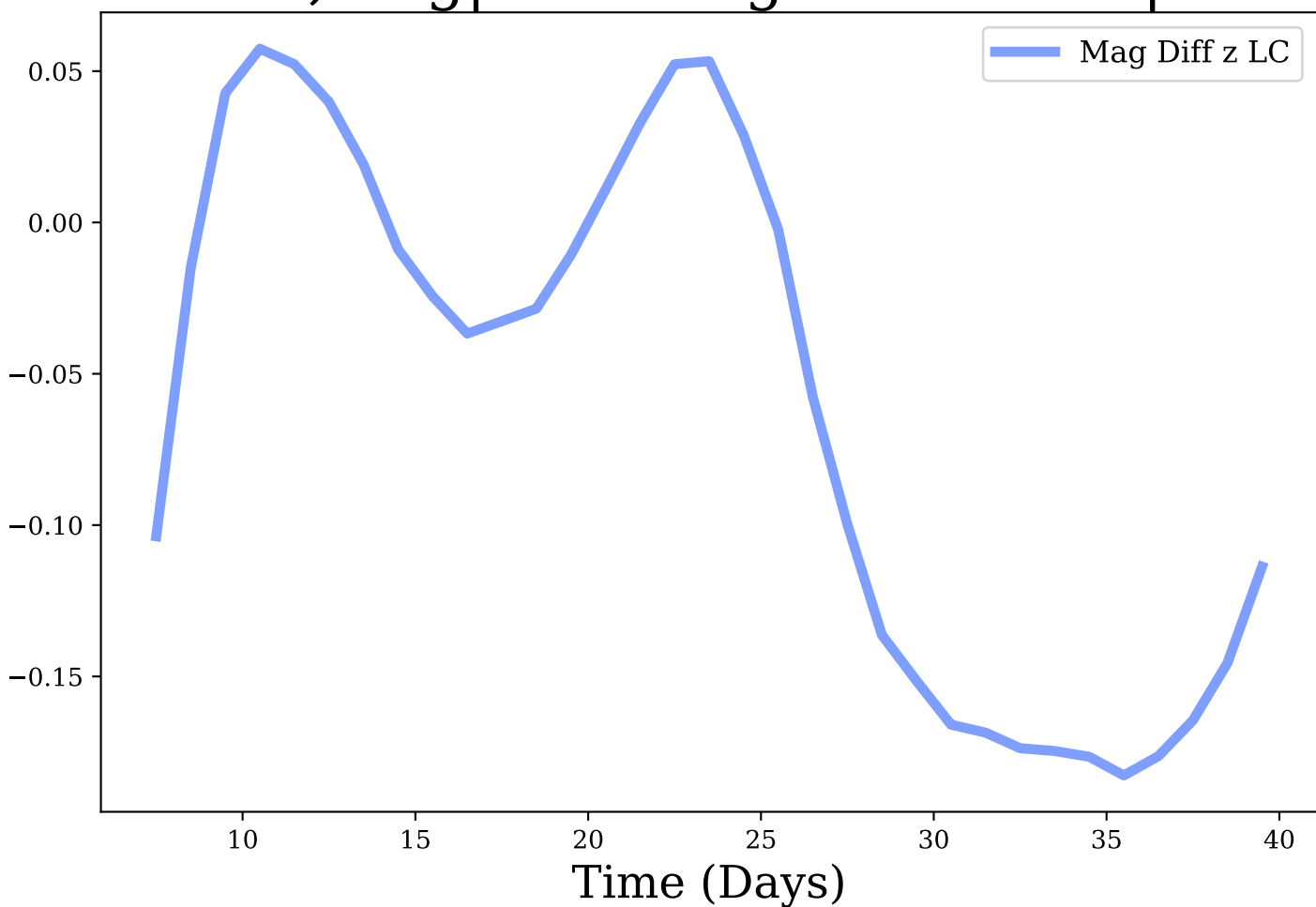
z-band, Avg|Max Mag Diff: -0.06 | 0.18
