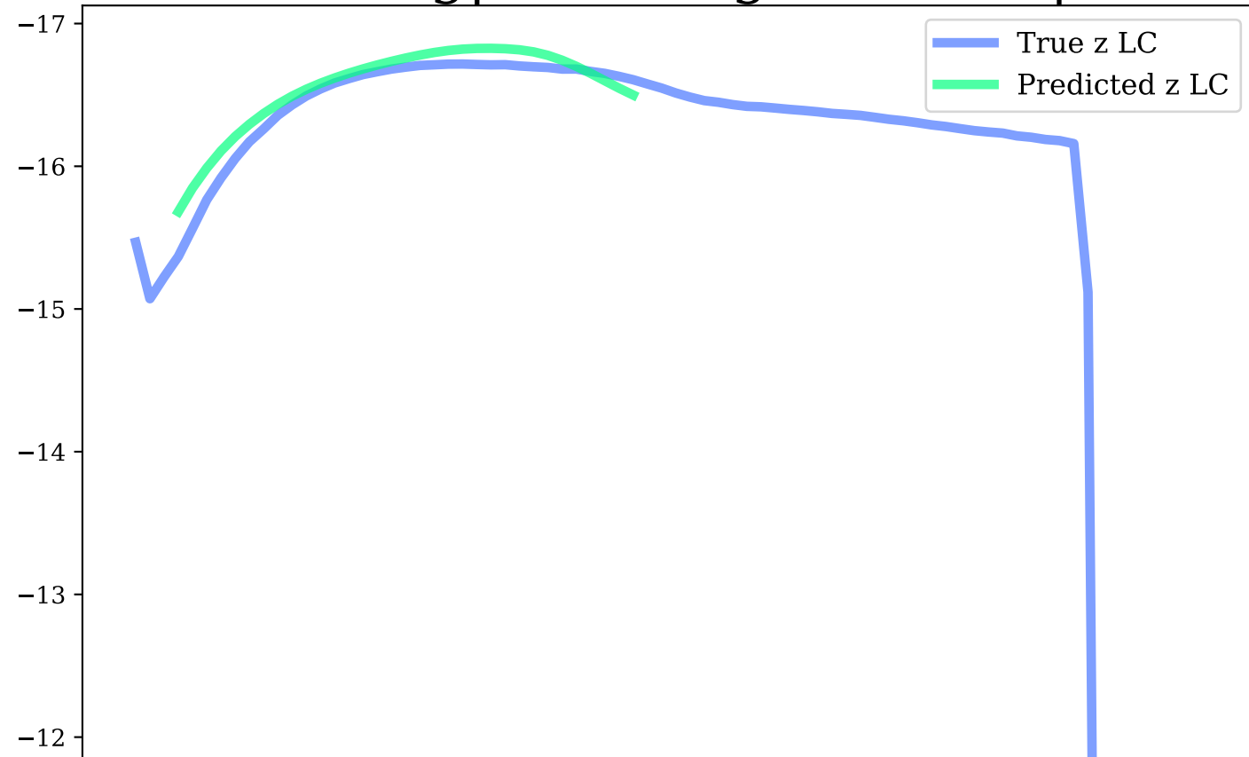
z-band, Avg|Max Mag Diff: 0.1 | 0.31
