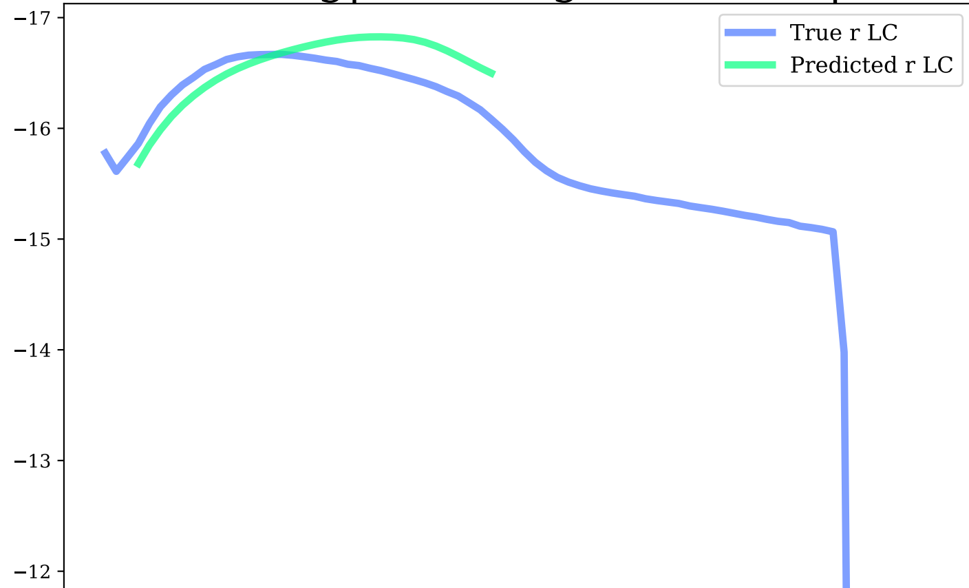
z-band, Avg|Max Mag Diff: 0.1 | 0.31
