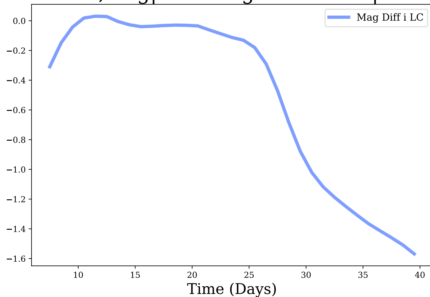
i-band, Avg|Max Mag Diff: -0.51 | 1.57
