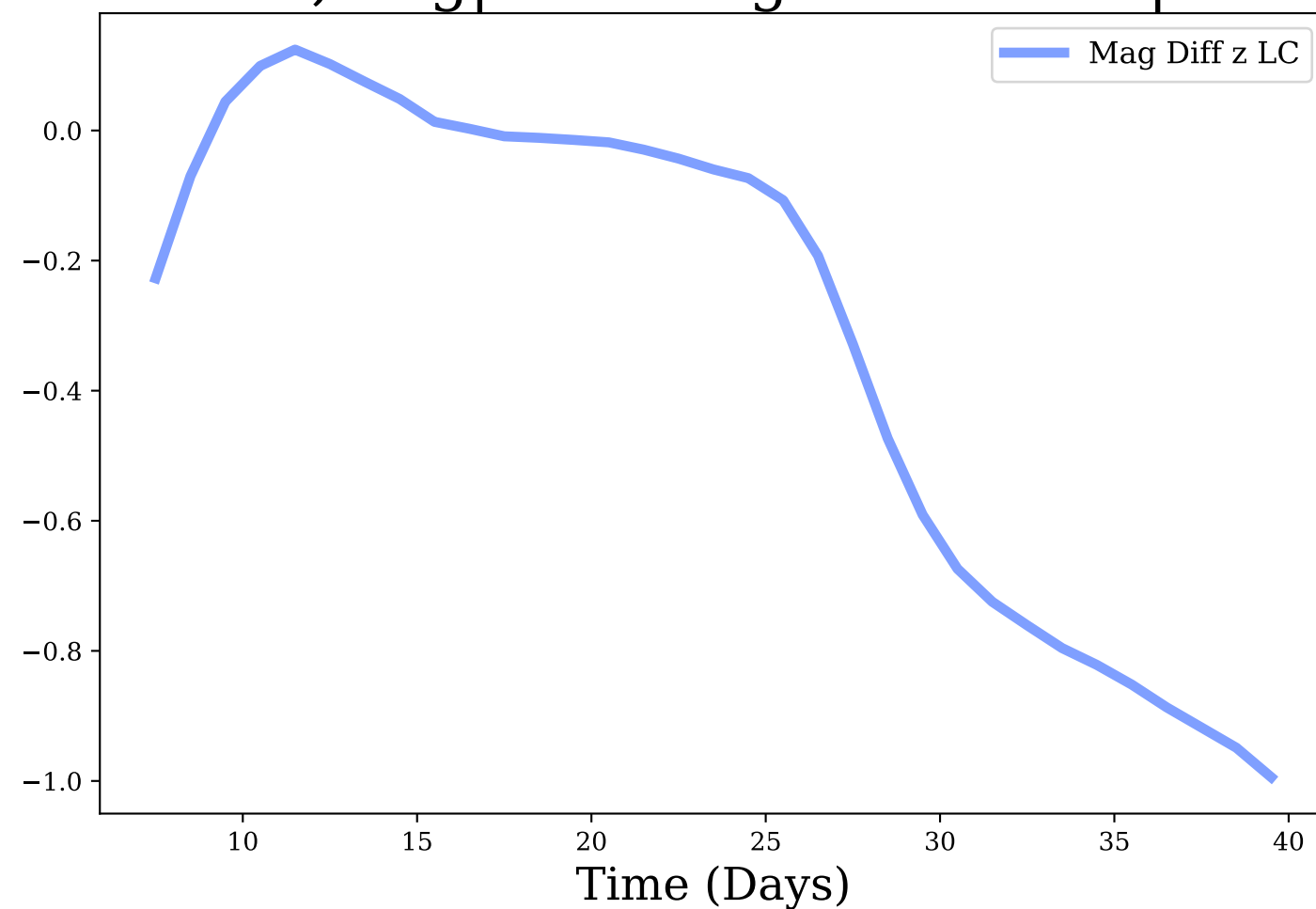
z-band, Avg|Max Mag Diff: -0.31 | 0.99
