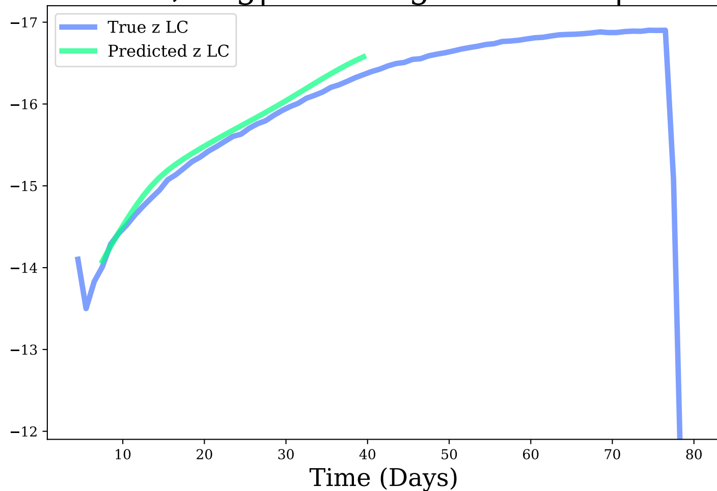
z-band, Avg|Max Mag Diff: 0.12 | 0.22
