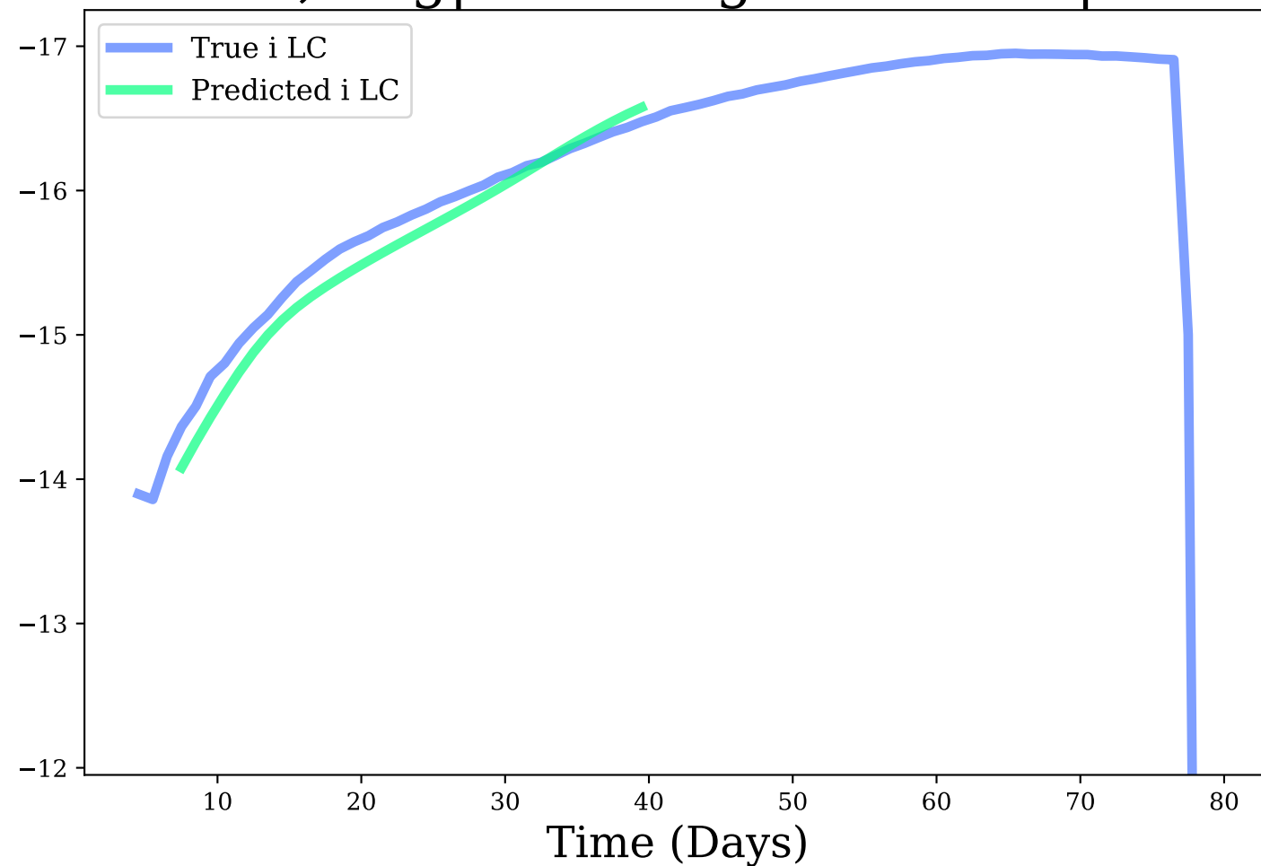
i-band, Avg|Max Mag Diff: 0.13 | 0.29
