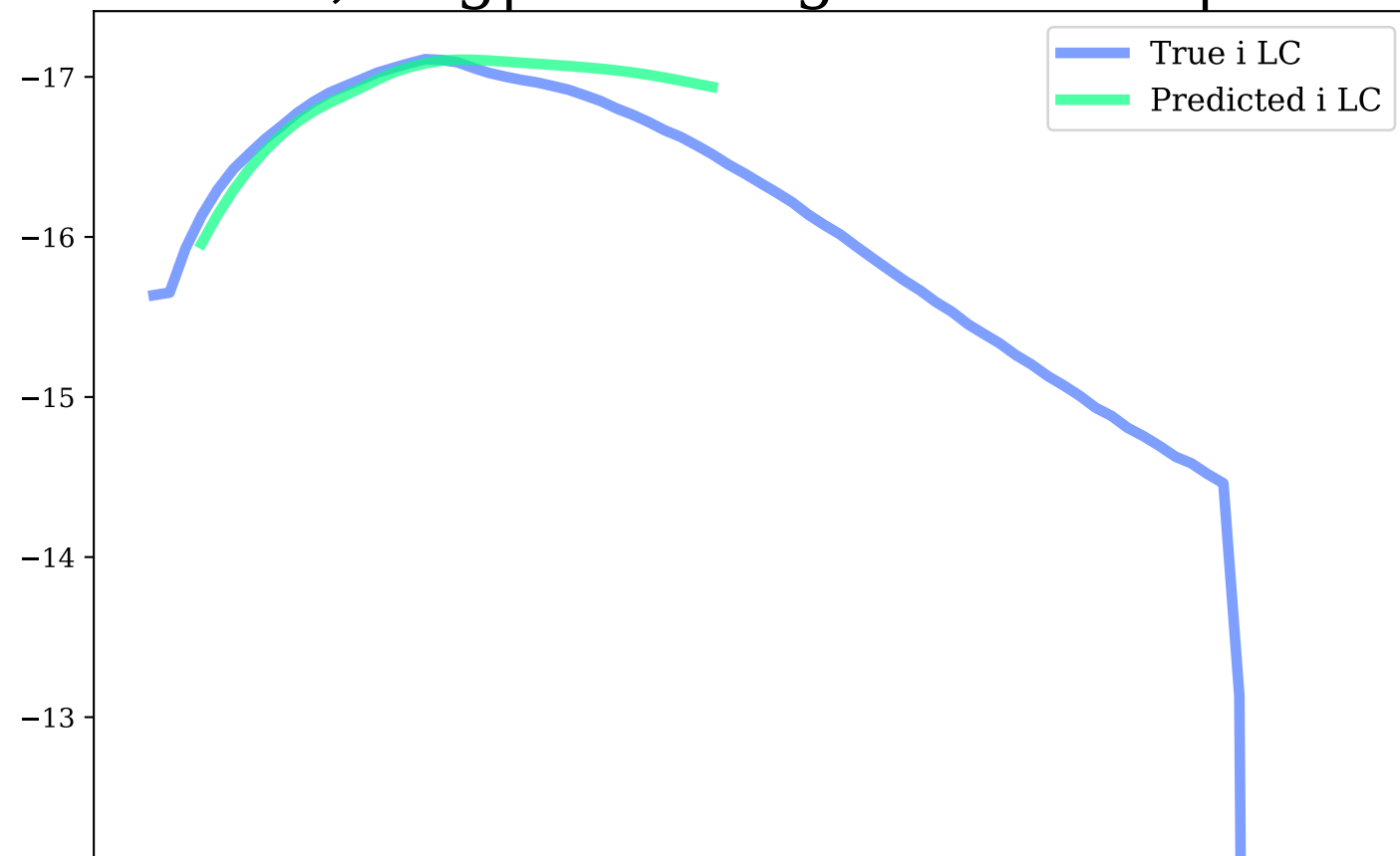
i-band, Avg|Max Mag Diff: 0.14 | 0.42
