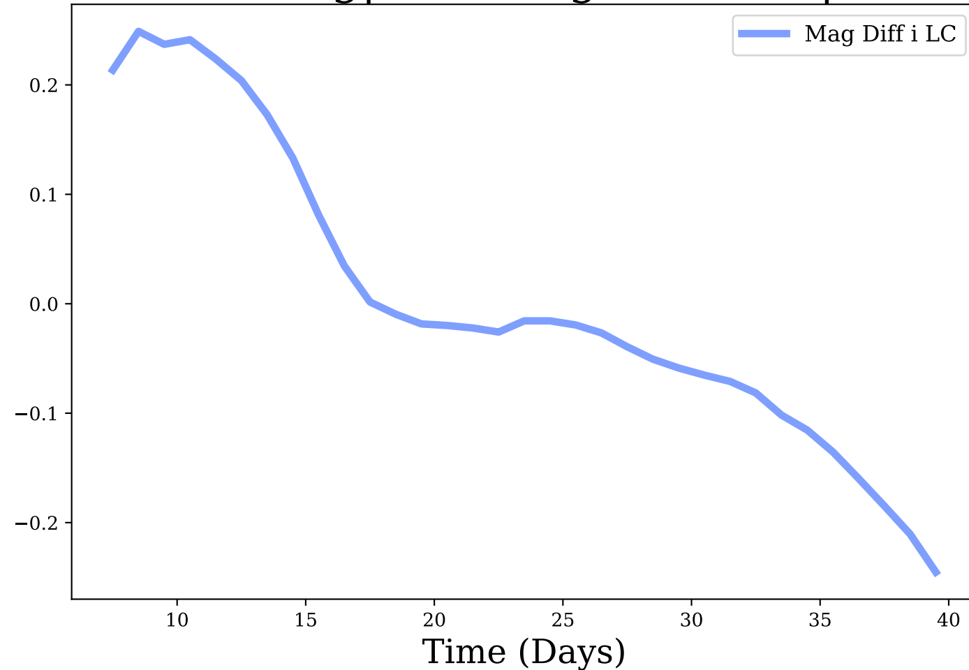
i-band, Avg|Max Mag Diff: 0.0 | 0.25
