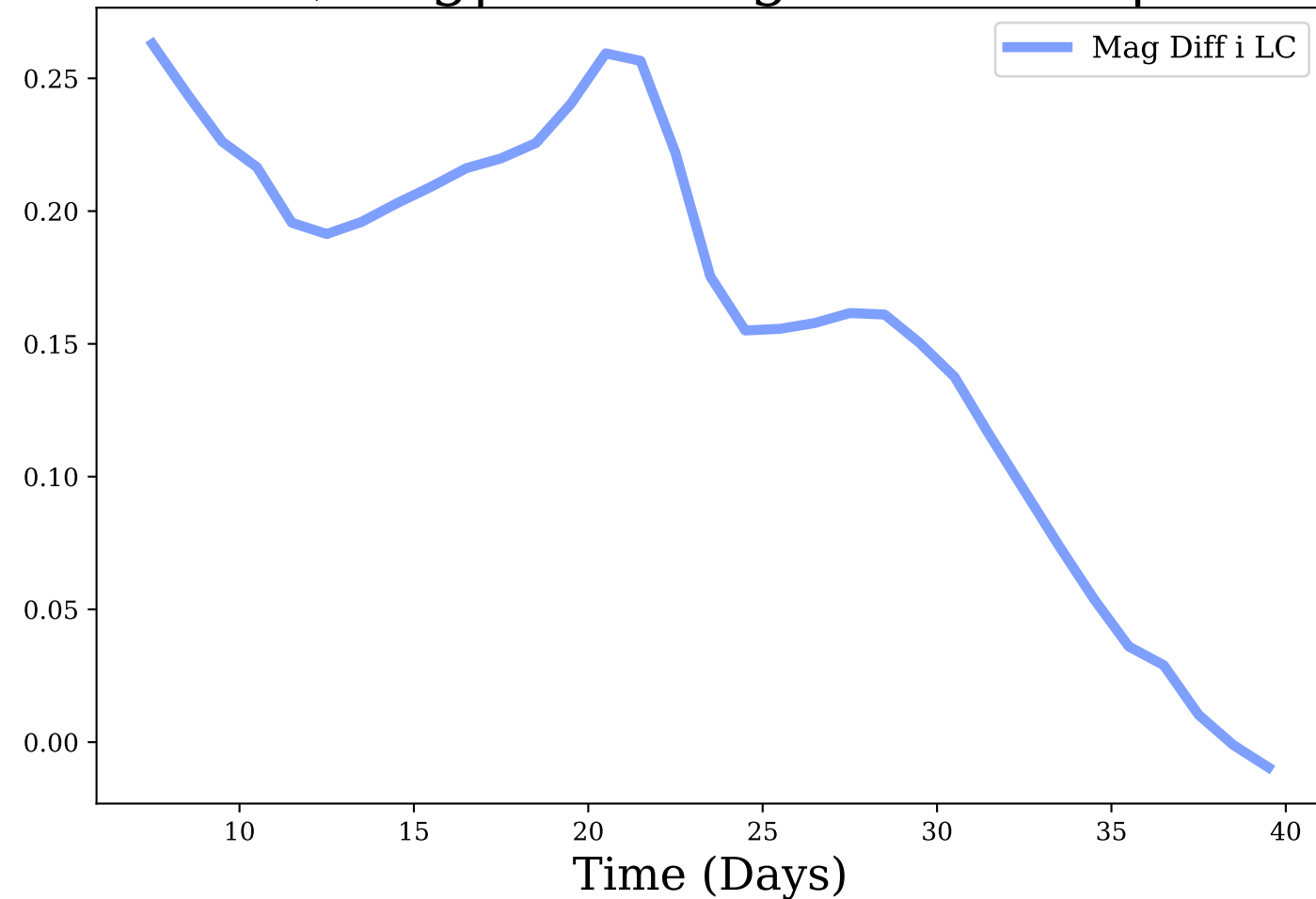
i-band, Avg|Max Mag Diff: 0.16 | 0.26
