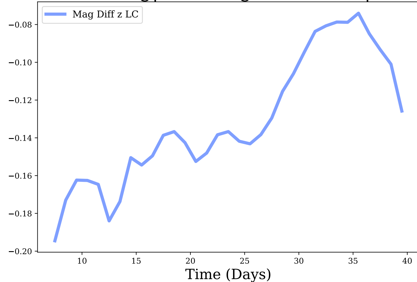
z-band, Avg|Max Mag Diff: -0.13 | 0.19
