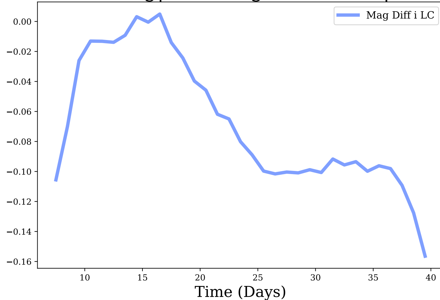
i-band, Avg|Max Mag Diff: -0.07 | 0.16
