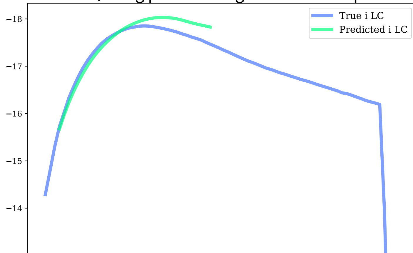
i-band, Avg|Max Mag Diff: 0.16 | 0.36
