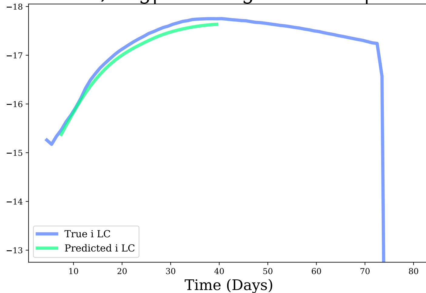
i-band, Avg|Max Mag Diff: 0.12 | 0.15
