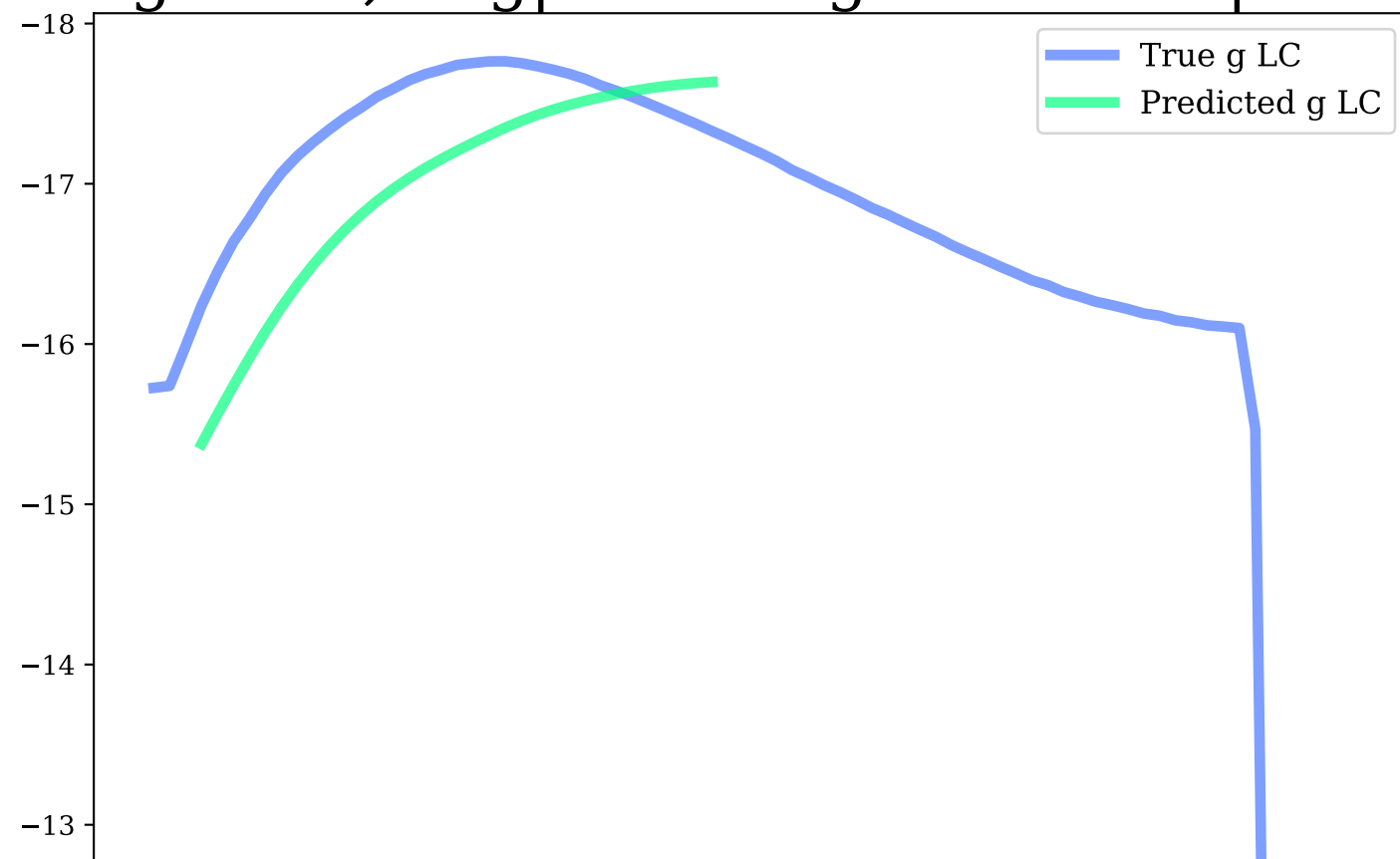
i-band, Avg|Max Mag Diff: 0.12 | 0.15
