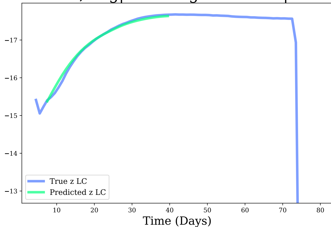
z-band, Avg|Max Mag Diff: 0.05 | 0.17
