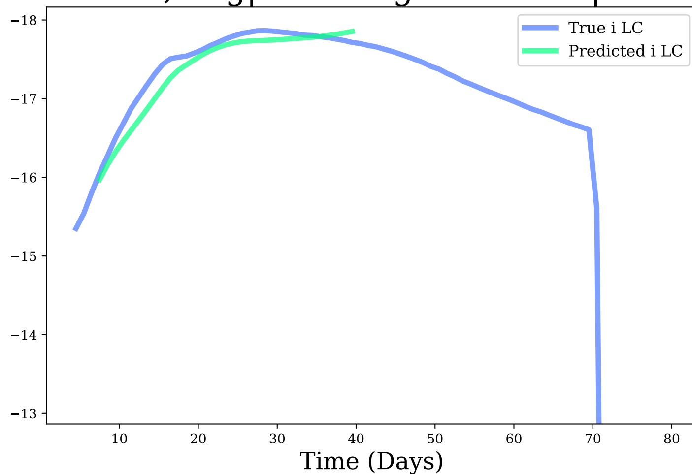
i-band, Avg|Max Mag Diff: 0.13 | 0.31
