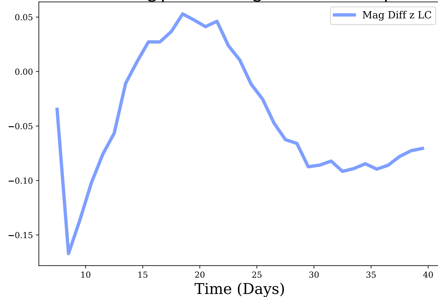
z-band, Avg|Max Mag Diff: -0.04 | 0.17
