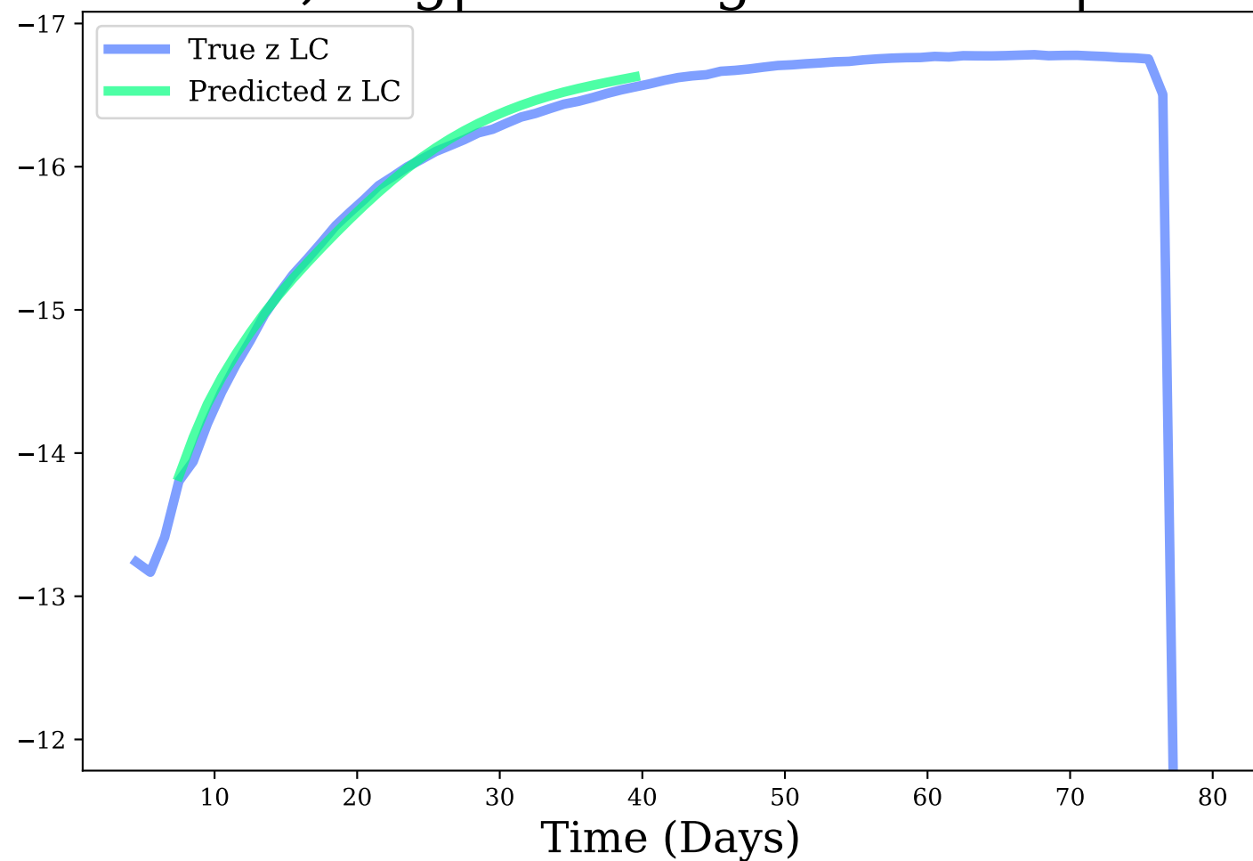
z-band, Avg|Max Mag Diff: 0.06 | 0.17
