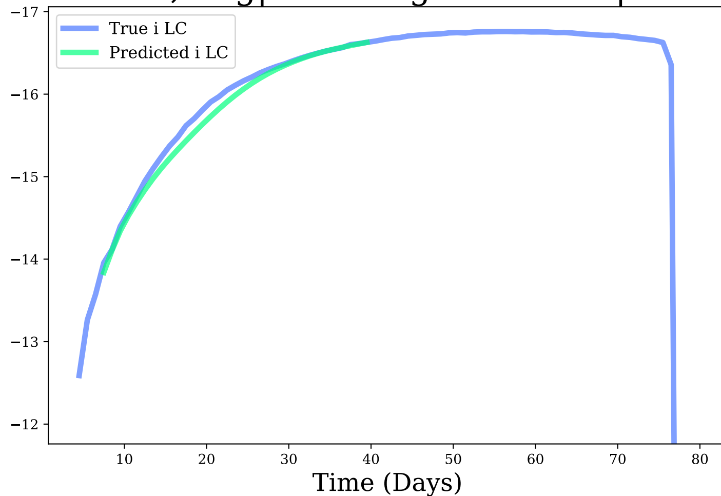
i-band, Avg|Max Mag Diff: 0.07 | 0.18
