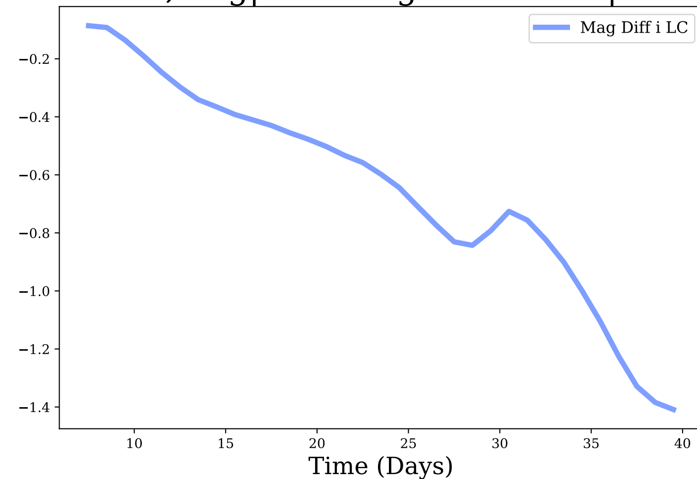
i-band, Avg|Max Mag Diff: -0.65 | 1.41
