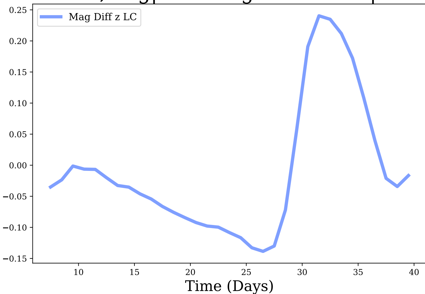
z-band, Avg|Max Mag Diff: -0.01 | 0.24
