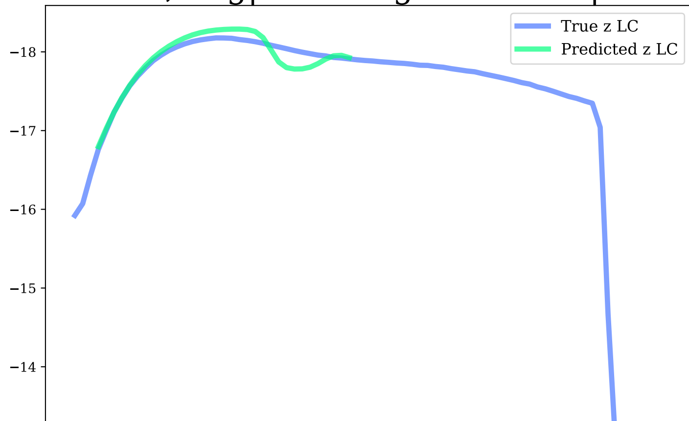
z-band, Avg|Max Mag Diff: 0.08 | 0.24
