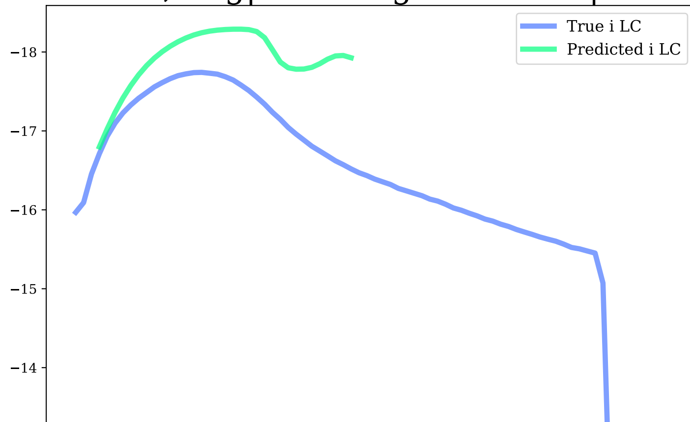
i-band, Avg|Max Mag Diff: 0.65 | 1.41
