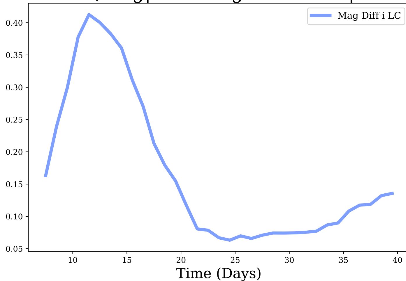
i-band, Avg|Max Mag Diff: 0.17 | 0.41
