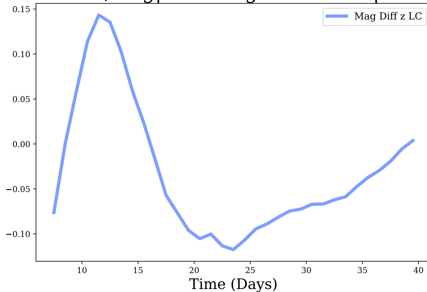
z-band, Avg|Max Mag Diff: -0.03 | 0.14
