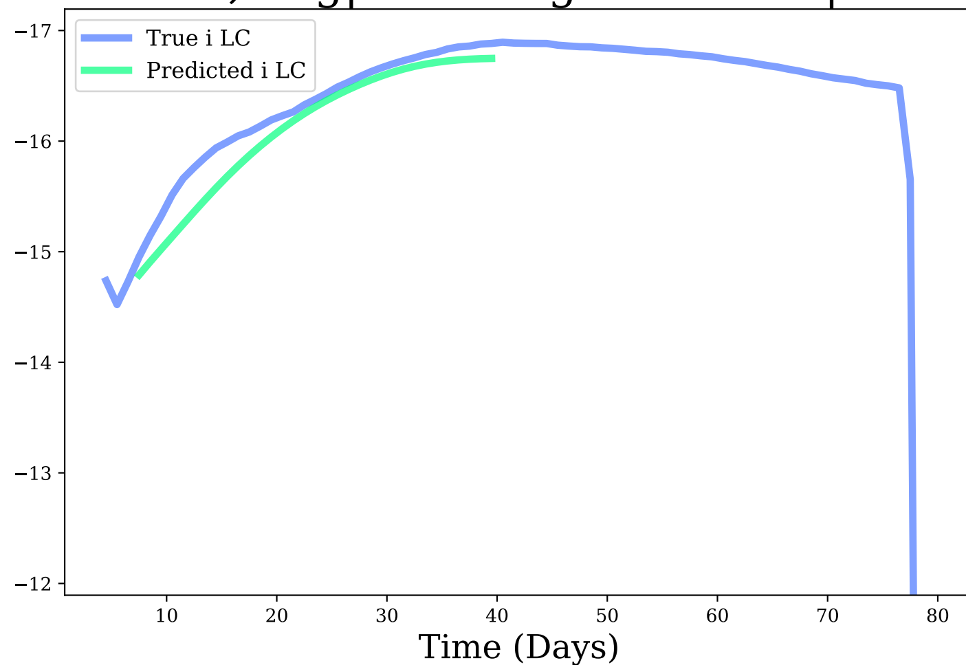
i-band, Avg|Max Mag Diff: 0.17 | 0.41
