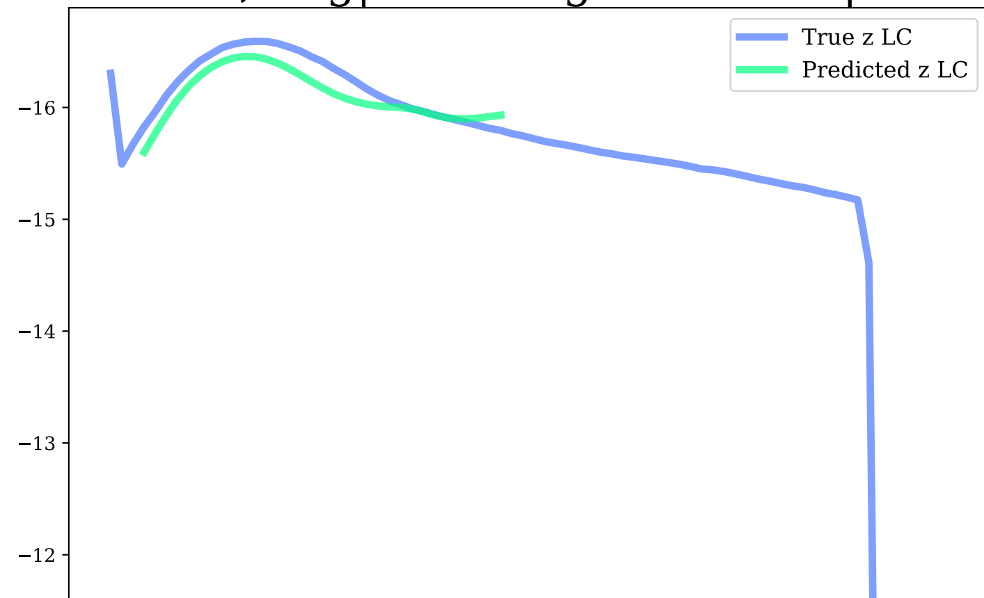
z-band, Avg|Max Mag Diff: 0.13 | 0.24
