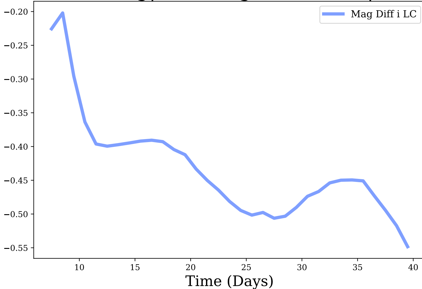
i-band, Avg|Max Mag Diff: -0.43 | 0.55
