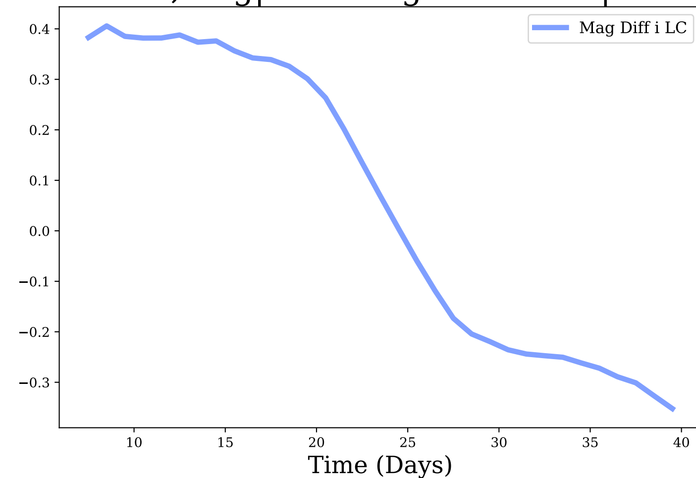
i-band, Avg|Max Mag Diff: 0.06 | 0.41
