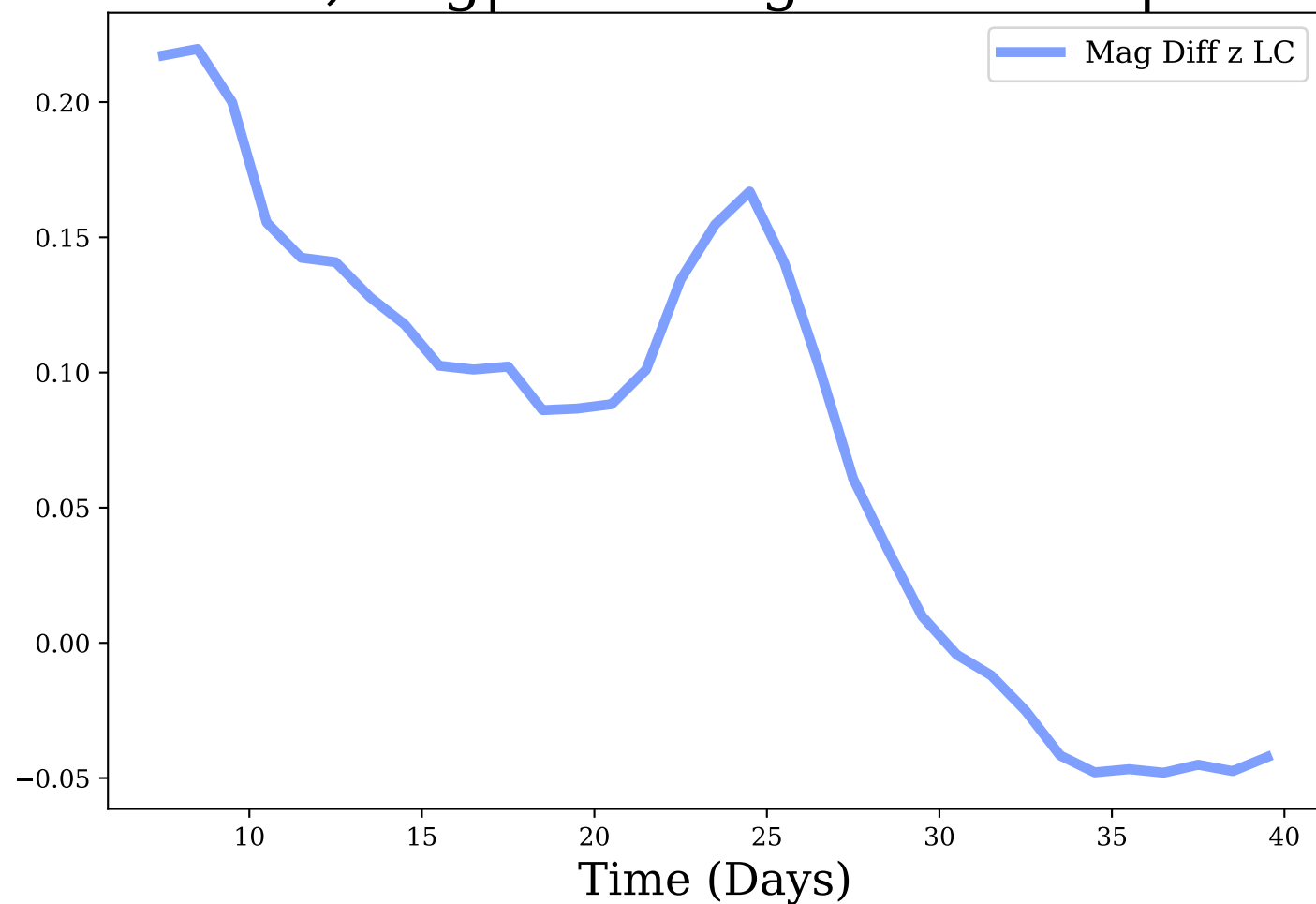
z-band, Avg|Max Mag Diff: 0.07 | 0.22
