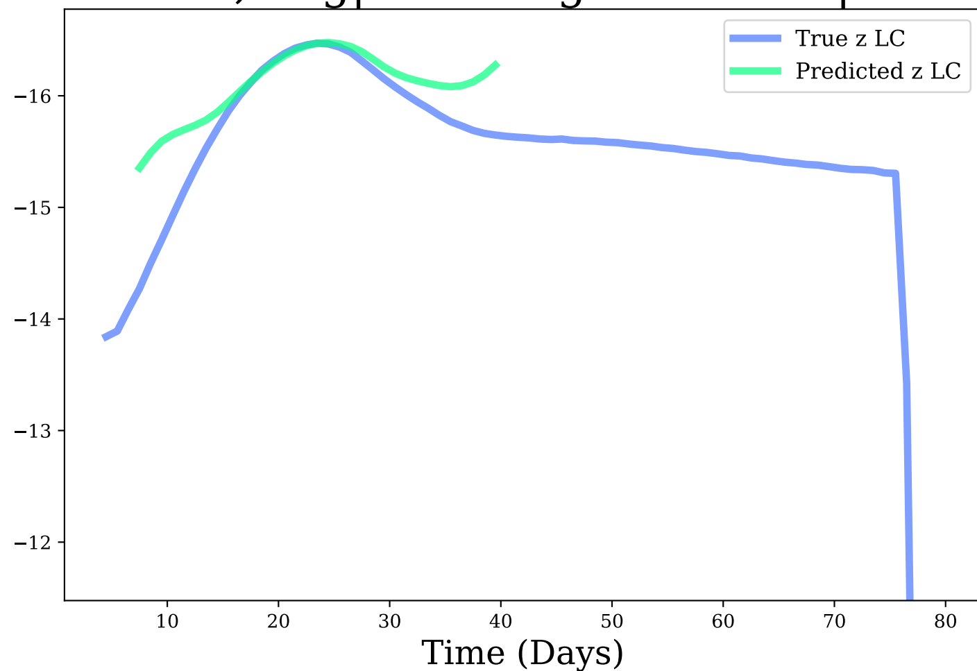
z-band, Avg|Max Mag Diff: 0.27 | 1.08
