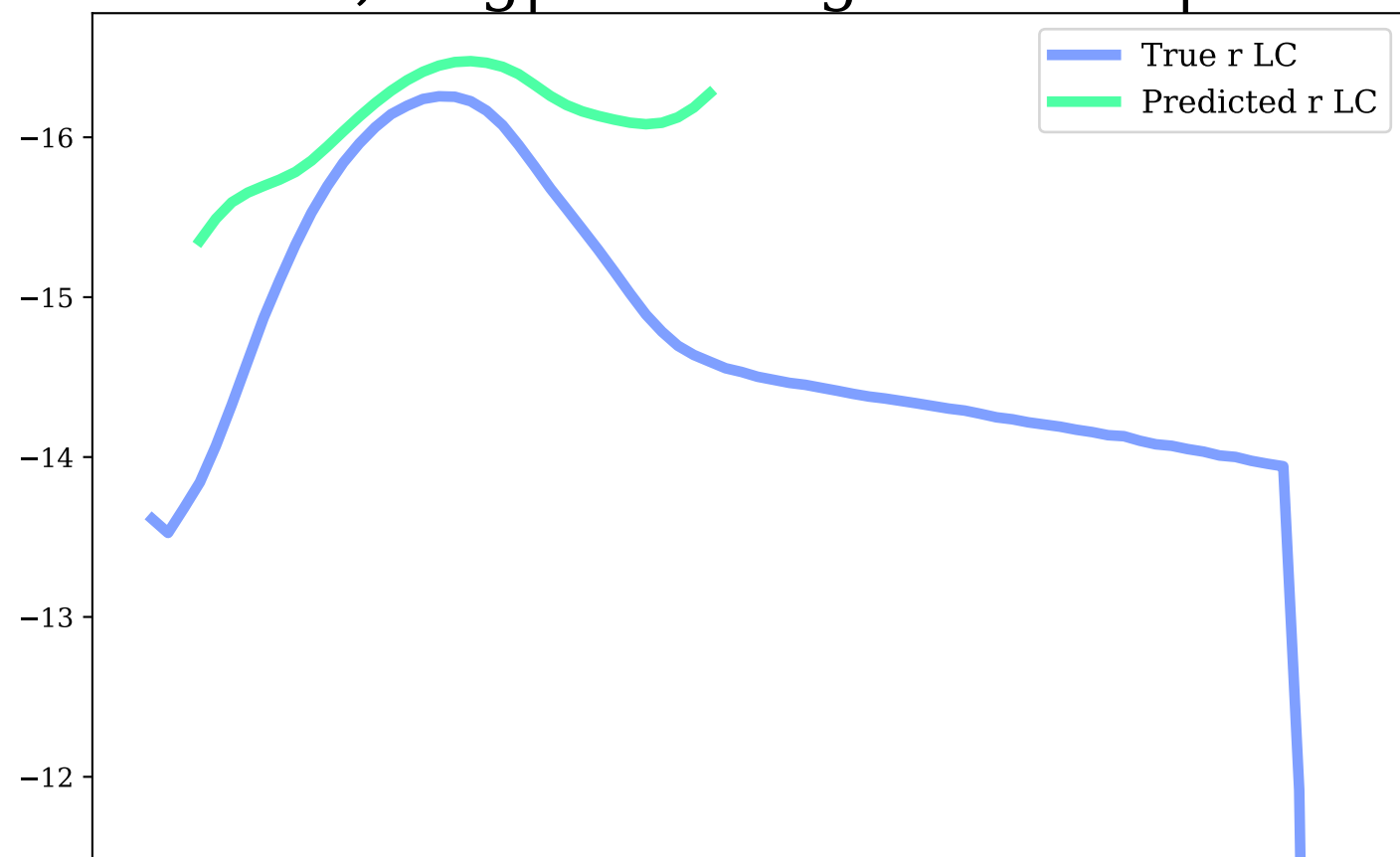
z-band, Avg|Max Mag Diff: 0.27 | 1.08
