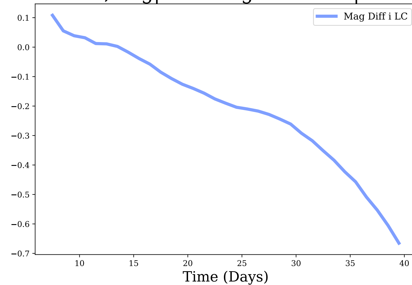
i-band, Avg|Max Mag Diff: -0.2 | 0.67
