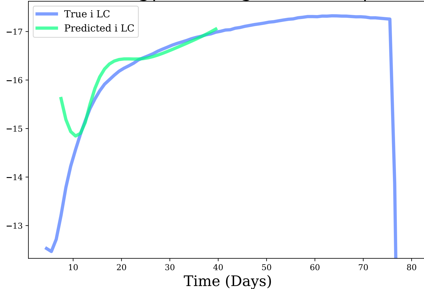
i-band, Avg|Max Mag Diff: 0.24 | 2.41
