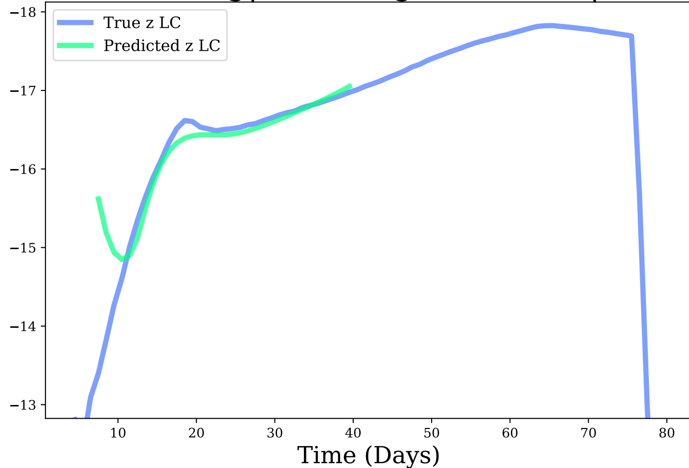
z-band, Avg|Max Mag Diff: 0.21 | 2.22
