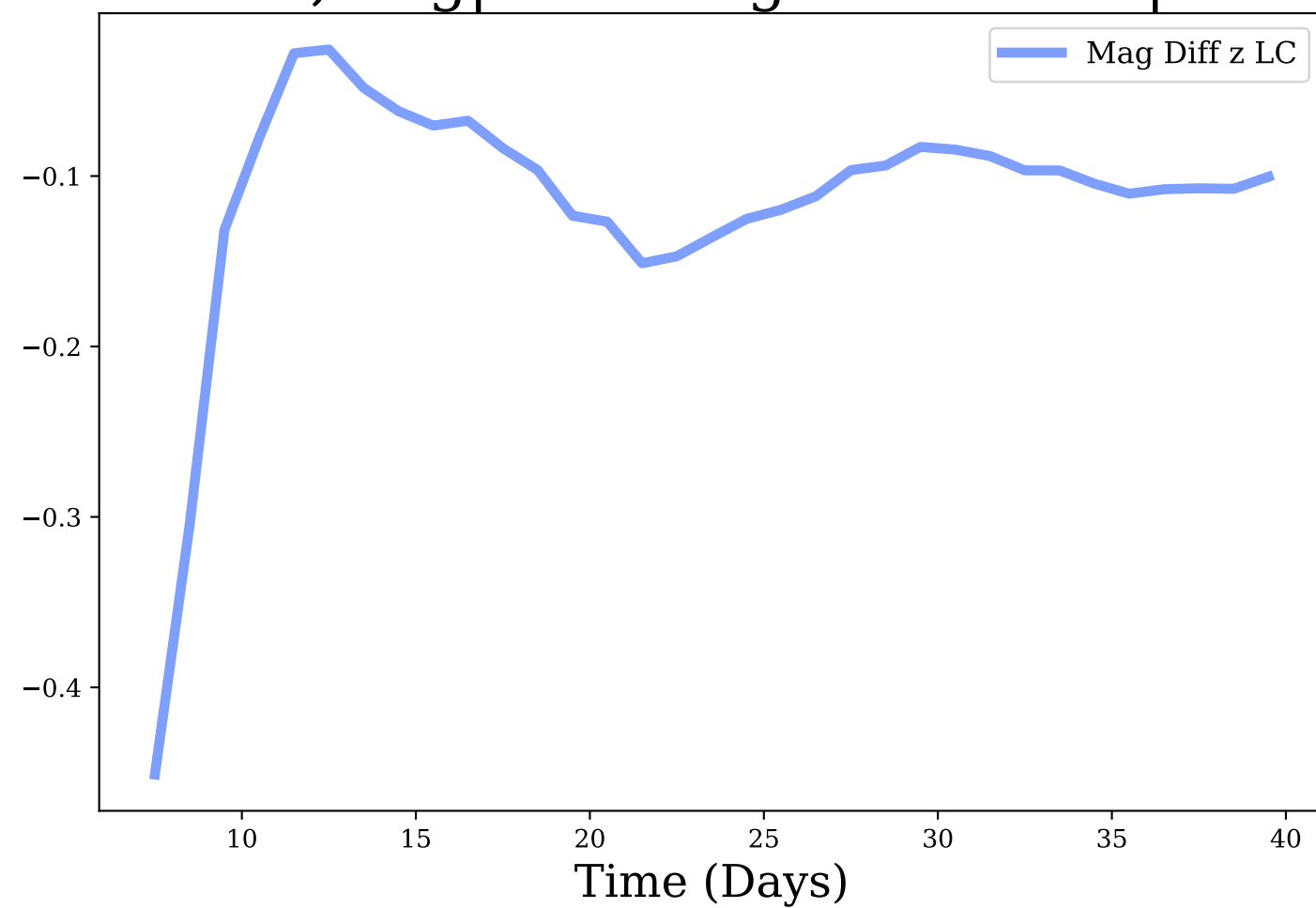
z-band, Avg|Max Mag Diff: -0.11 | 0.45
