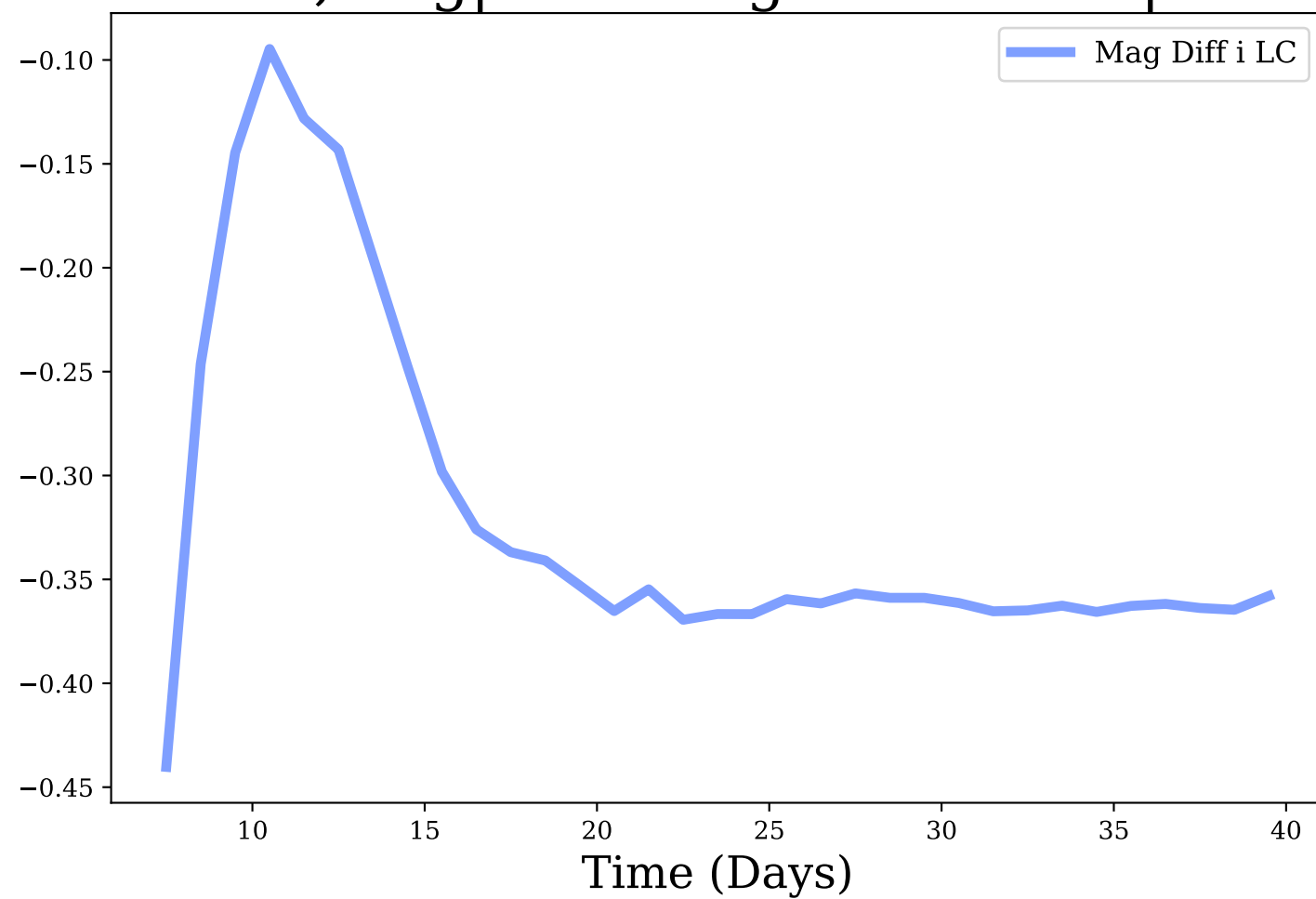
i-band, Avg|Max Mag Diff: -0.32 | 0.44
