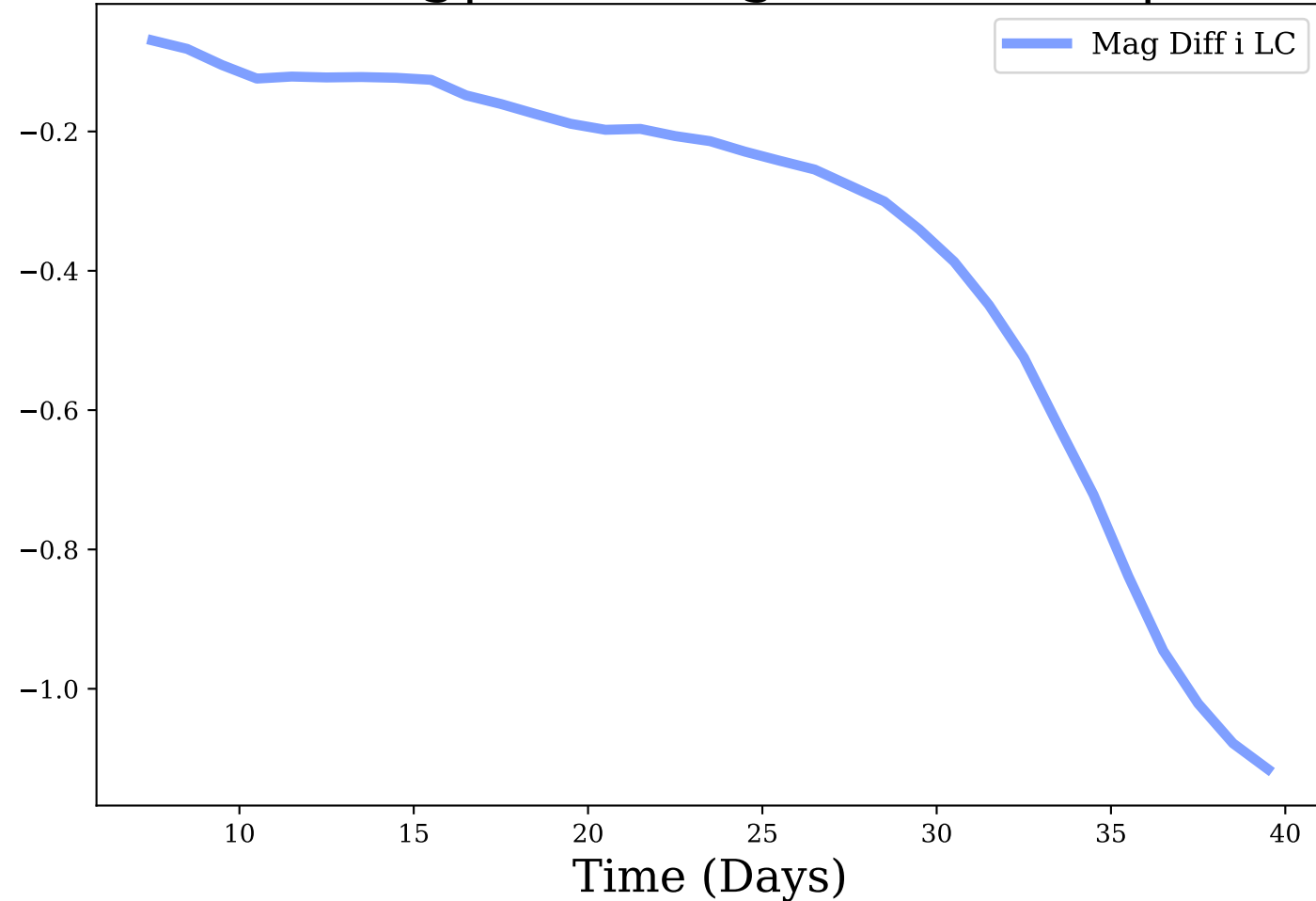
i-band, Avg|Max Mag Diff: -0.36 | 1.12
