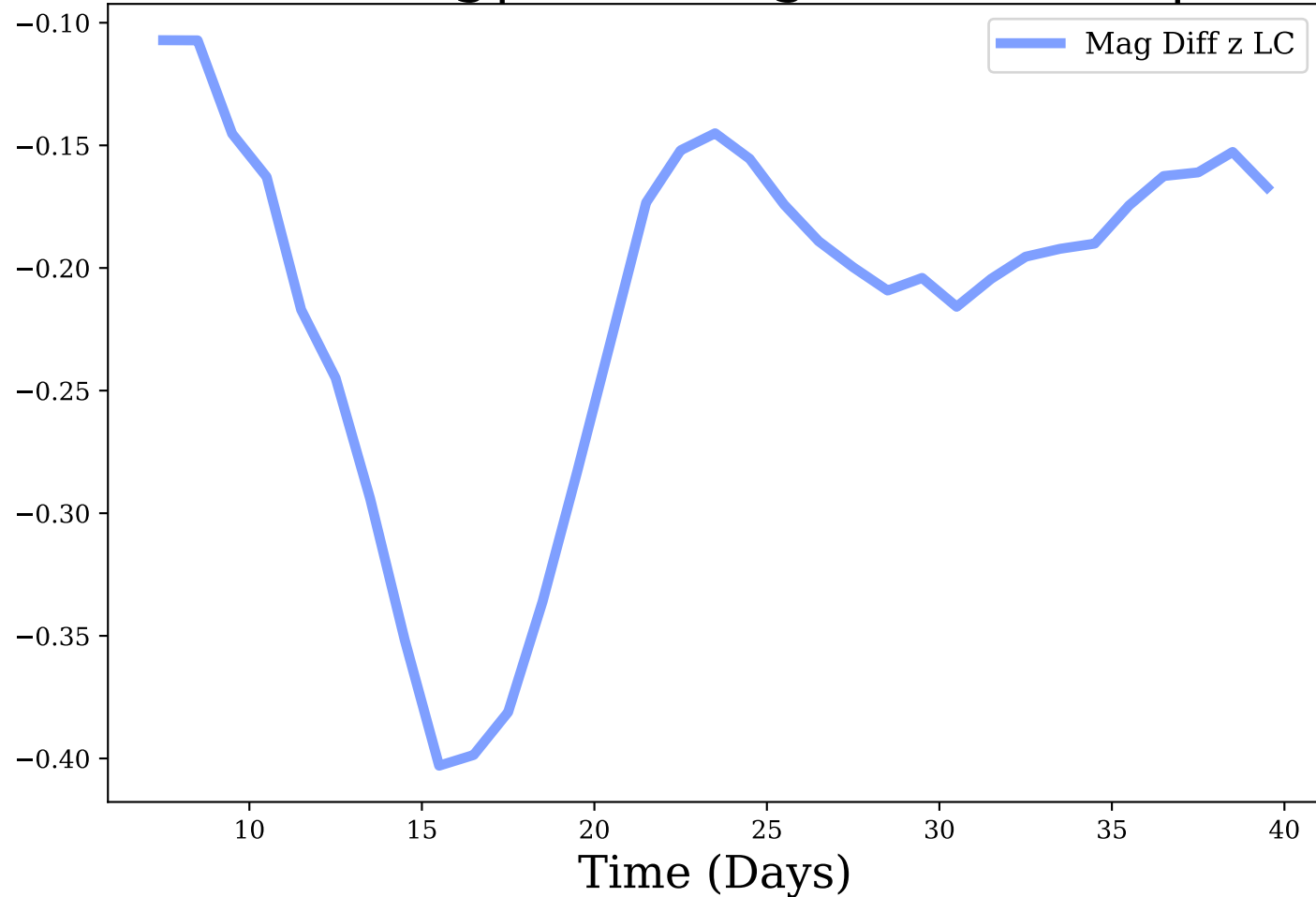
z-band, Avg|Max Mag Diff: -0.21 | 0.4
