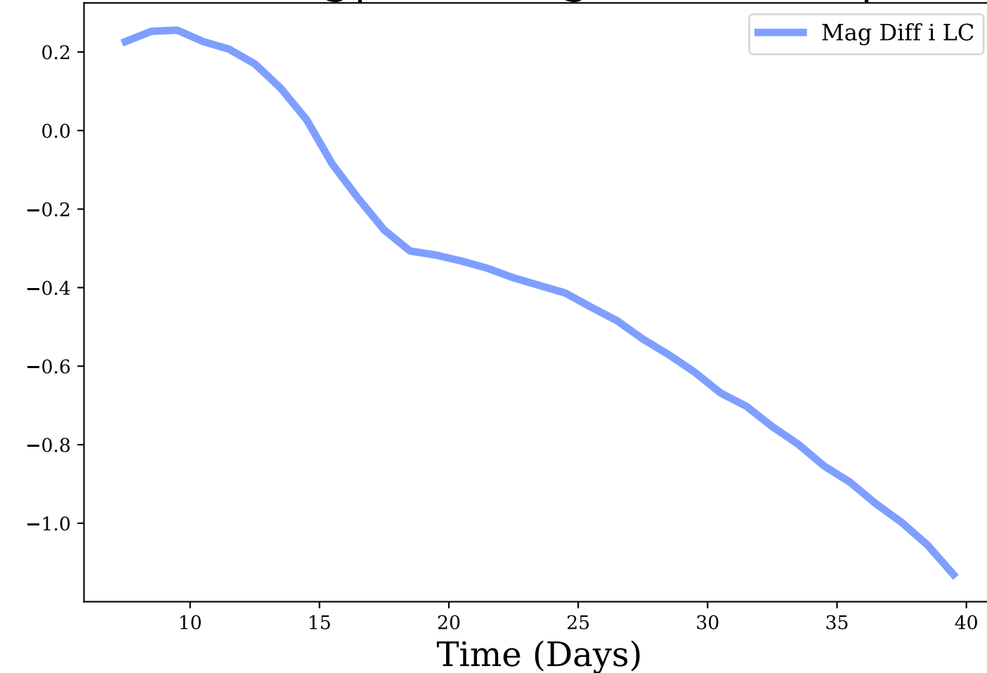
i-band, Avg|Max Mag Diff: -0.39 | 1.13
