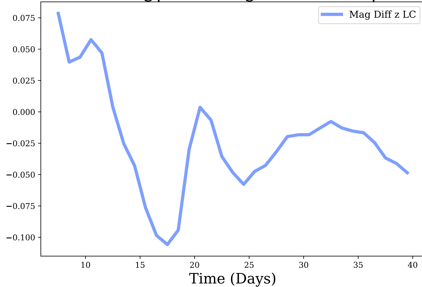
z-band, Avg|Max Mag Diff: -0.02 | 0.11
