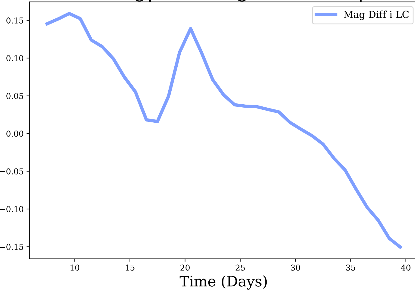
i-band, Avg|Max Mag Diff: 0.03 | 0.16
