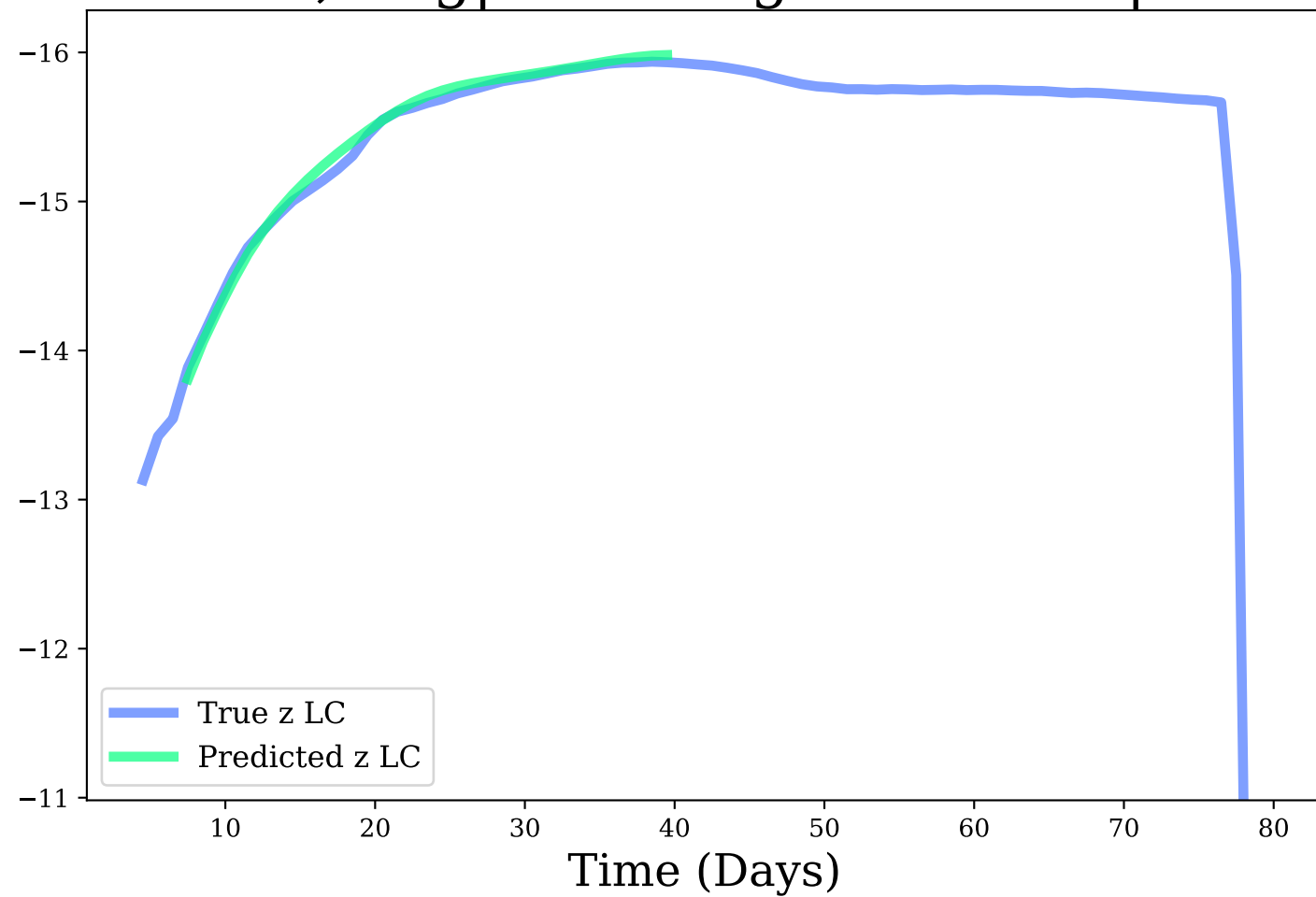
z-band, Avg|Max Mag Diff: 0.04 | 0.11
