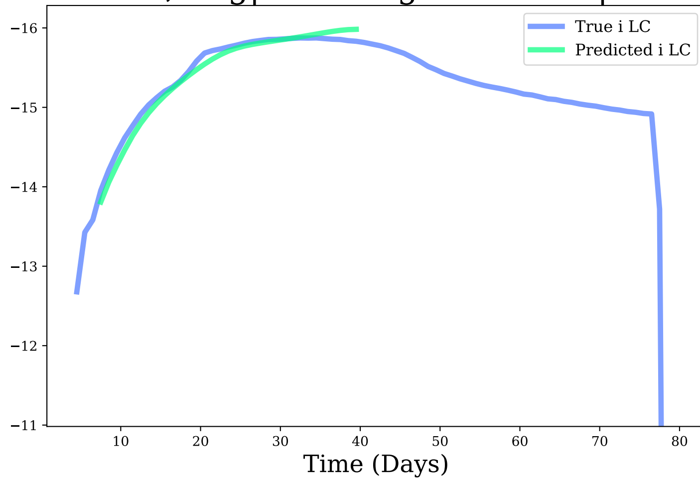
i-band, Avg|Max Mag Diff: 0.08 | 0.16
